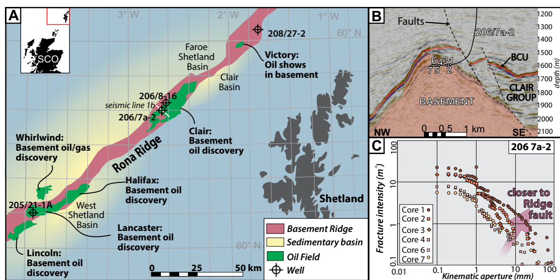
Figure 1. A: Simplified map showing location of Rona Ridge basement, oil fields, and wells referred to in this study (offshore Shetland, UK). SCO—Scotland. Mapped extent of the Clair Field includes the Devonian part of the reservoir (Clair Group). B: Northwest-southeast seismic reflection profile through the Clair Field (line of section shown in A) showing location of basement ridge, Clair Group, and base-Cretaceous unconformity (BCU; after Holdsworth et al., 2018). Position of 206/7a-2 well (drilled by Elf U.K. Ltd. in 1991) and associated cores shown in C are also shown. Note that the main Ridge fault here lies on the southeast side of the basement ridge; in other areas, such as Lancaster, equivalent structures lie on the northwest side (Trice, 2014); i.e., polarity of faulting changes along strike. C: Plot using approach of Ortega et al. (2006) showing how both fracture intensity (no. fractures/m) and kinematic aperture increase by almost an order of magnitude in the 206/7a-2 cores closer to Ridge fault. Slopes of distributions are consistently close to -1 .
