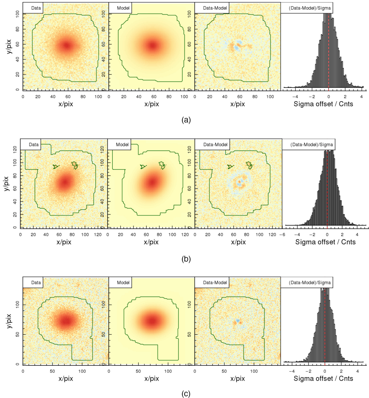
Figure 8. Example of PROFIT single Sérsic fits to VST KiDS r -band images of the galaxies shown in Fig. 1. Column one shows the data image, column two shows the selected model, column three shows a difference image, and column four shows a histogram of the residuals. The green contour indicates the fitting region derived from a Source Extractor image segmentation.
