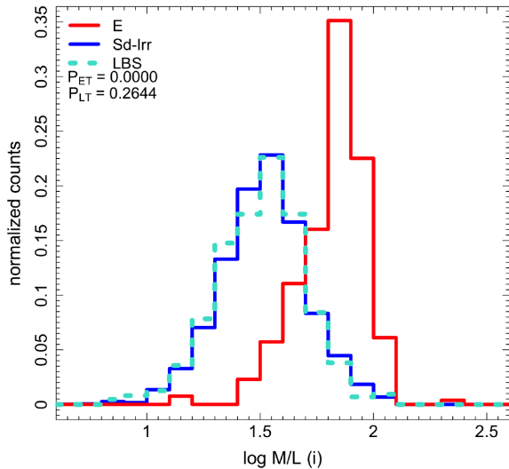
Figure 5. Distribution of LBS i -band mass-to-light ratios compared to those of Sd-Irr and low-mass E galaxies, illustrating that LBS and Sd-Irr mass-to-light ratio distributions are indistinguishable. The legend indicates p-values derived from K-S tests comparing the LBS property distribution to those of low-mass E ( P_{ET} ) and Sd-Irr ( P_{LT} ) populations.
