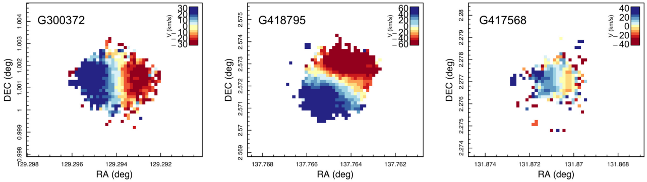
Figure 13. SAMI emission line velocity maps derived from the analysis described by Green et al. (2018) and Medling et al. (2018). The left and middle panels show examples of LBS galaxies with velocity fields that display extended, regular rotation well fit by the symmetric rising rotation curve form used here, while the far right panel shows an example of an LBS velocity field that is poorly fit with this rotation curve form. Note that the category of galaxies that are poorly fit by a symmetric rising rotation curve (and for which we cannot obtain a reliable characteristic rotation velocity with this method) includes both objects with some evidence of disturbed rotation (as in the far right panel above) and those with no apparent rotation signature. We omit spaxels with large measured velocity errors ( >15 \text{ km s}^{-1} ) from the plotted maps.
