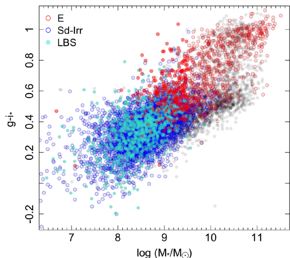
Figure 2. GAMA Visual Morphology sample in colour versus stellar mass space, where g - i_* is the intrinsic (corrected for internal dust extinction) g - i colour from the SED modelling of Taylor et al. (2011). Stellar mass estimates are also derived from Taylor et al. (2011). Light grey points indicate the full sample distribution with coloured points indicating the E, Sd-Irr, and LBS classes. The subsample of ‘low-mass E’ galaxies is indicated in filled red points.
