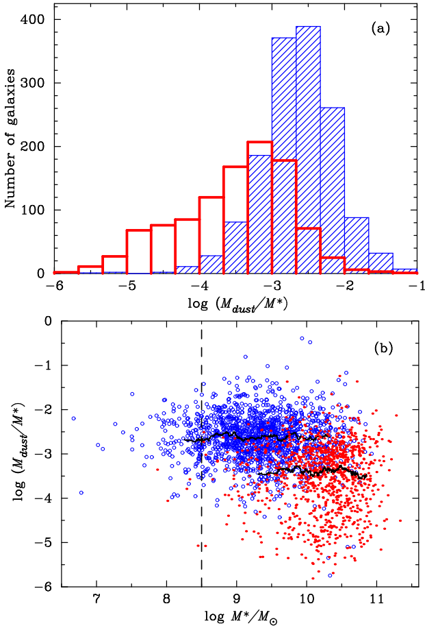
Figure 8. (a) The distribution of dust-to-stellar-mass ratio for the blue ( hatched ) and red ( solid ) spiral galaxies, respectively. The specific production of dust is lower in the red spiral galaxies as compared to the blue spiral galaxies. (b) The DTS ratio is shown as a function of M^* for the two colour-selected samples of spiral galaxies. Symbols are same as in Fig. 4. The horizontal solid horizontal lines represent the median trends in the two colour-selected samples, while the vertical dashed line represents the limiting stellar mass at the maximum redshift of our sample.
