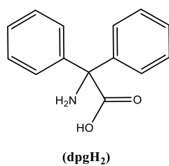
Scheme 1. 2,2'-Diphenylglycine (dpgH 2 ) and benzilic acid (2,2'-diphenylglycolic acid, benzH).
