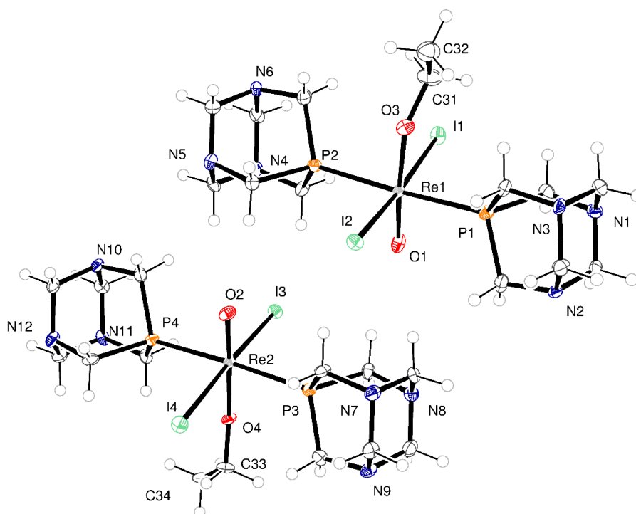
Figure 2. Molecular structure of [\text{ReO}(\text{OEt})\text{I}_2(\text{PTA})_2] ( 2 ). Selected bond lengths ( \text{\AA} ) and angles ( ^\circ ): \text{Re}(1)\text{-O}(1) 1.706(5), \text{Re}(1)\text{-O}(3) 1.906(5), \text{Re}(1)\text{-I}(1) 2.8117(5), \text{Re}(1)\text{-I}(2) 2.7450(5), \text{Re}(1)\text{-P}(1) 2.4673(17), \text{Re}(1)\text{-P}(2) 2.4523(17); \text{O}(1)\text{-Re}(1)\text{-O}(3) 172.6(2), \text{P}(2)\text{-Re}(1)\text{-P}(1) 176.27(6), \text{O}(1)\text{-Re}(1)\text{-I}(2) 95.59(16), \text{C}(31)\text{-O}(3)\text{-Re}(1) 146.9(4), \text{O}(3)\text{-C}(31)\text{-C}(32) 111.9(6). \text{Re}(2)\text{-O}(2) 1.705(5), \text{Re}(2)\text{-O}(4) 1.906(5), \text{Re}(2)\text{-I}(3) 2.7519(5), \text{Re}(2)\text{-I}(4) 2.8080(5), \text{Re}(2)\text{-P}(3) 2.4555(17), \text{Re}(2)\text{-P}(4) 2.4631(17); \text{O}(2)\text{-Re}(2)\text{-O}(4) 174.3(2), \text{P}(3)\text{-Re}(2)\text{-P}(4) 176.24(6), \text{O}(2)\text{-Re}(2)\text{-I}(3) 94.42(15), \text{C}(33)\text{-O}(4)\text{-Re}(2) 152.0(4), \text{O}(4)\text{-C}(33)\text{-C}(34) 111.2(5).
