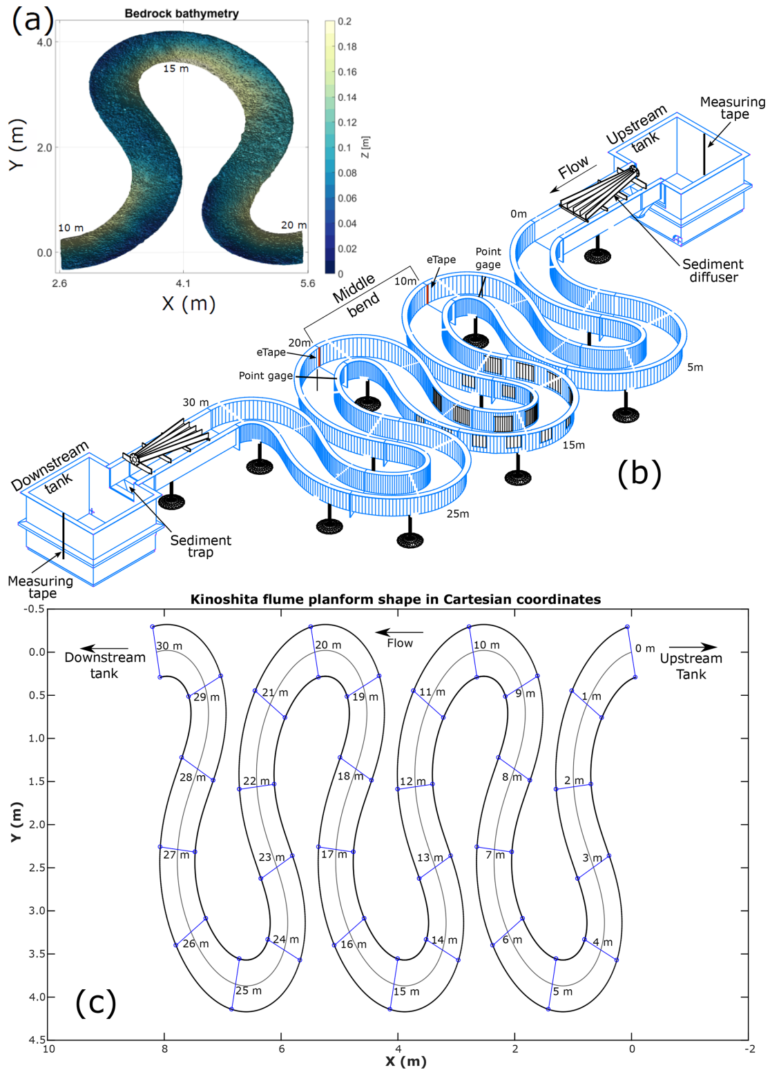
Figure 2. (a) Bedrock bathymetry built inside the Kinoshita flume. Streamwise locations 10, 15, and 20 m are indicated; (b) 3-D rendering of the Kinoshita flume showing the location of tank measuring tapes, point gages, eTapes, a sediment trap and sediment diffuser, flow direction, and the middle bend where all measurements were made. (c) Kinoshita shape with streamwise stations indicated. Flow direction from right to left.
