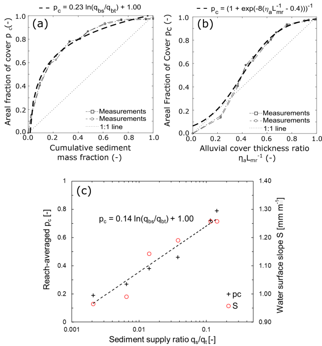
Figure 5. (a) Relation between the areal fraction of alluvial cover and cumulative sediment mass fraction for bedrock slab; the total mass added to the slab was 646 g and all increments are shown in Supplement S1. (b) Relation between the areal fraction of alluvial cover and the ratio between alluvial thickness and bedrock macro-roughness for bedrock slab. (c) Relation between the reach-averaged areal fraction of alluvial cover and sediment supply ratio for the Kinoshita flume and corresponding water surface slopes as a function of sediment supply ratio.
