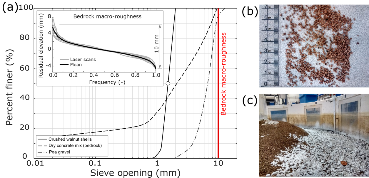
Figure 3. (a) Grain size distributions for the alluvium (crushed walnut shells), dry concrete mix used to build the bedrock, and the pea gravel underlying the bedrock basement. Insert shows residual elevations of as-built bedrock bed, measured with laser scans at different cross sections inside the Kinoshita flume. Mean macro-roughness ( \sim 10 mm) is also indicated in the main plot. (b) Image of crushed walnut shells with a ruler for scale and (c) bedrock bed partially covered with alluvium inside the Kinoshita flume.
