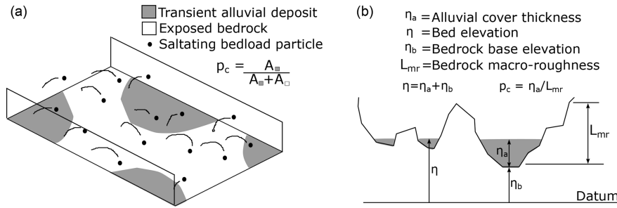
Figure 1. Schematic representations of (a) the fraction of exposed bedrock showing surface areal cover (Sklar and Dietrich, 2004) and (b) a cross section illustrating the filling of a rough bedrock surface with alluvium (Zhang et al., 2015).
