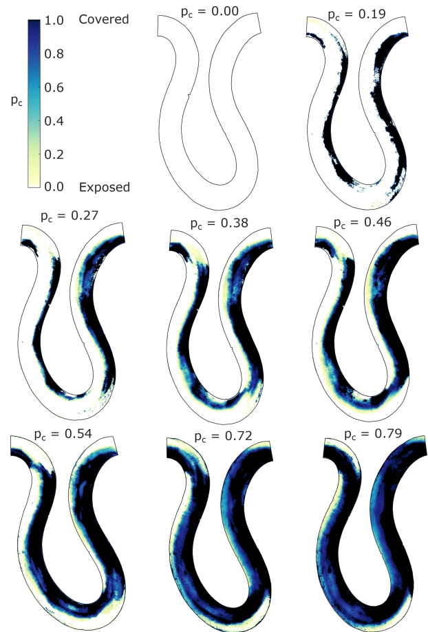
Figure 8. Maps of spatiotemporal averages of the areal fraction of alluvial cover for all experimental conditions.
