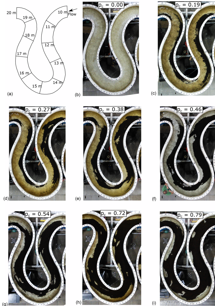
Figure 6. Images of the middle bend of the Kinoshita flume corresponding to an instant during each of the eight different areal alluvial cover conditions. The volume of sediment in the system grows from top to bottom and left to right. (a) Diagram showing the flow direction with cross sections indicating the streamwise locations along the middle bend of the flume.
