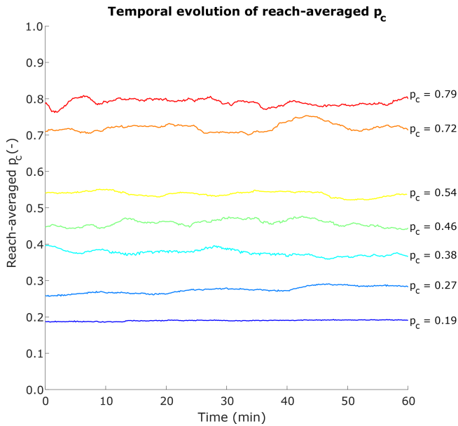
Figure 7. Temporal evolution of the reach-averaged areal fraction of alluvial cover for all experimental conditions that had alluvium.
