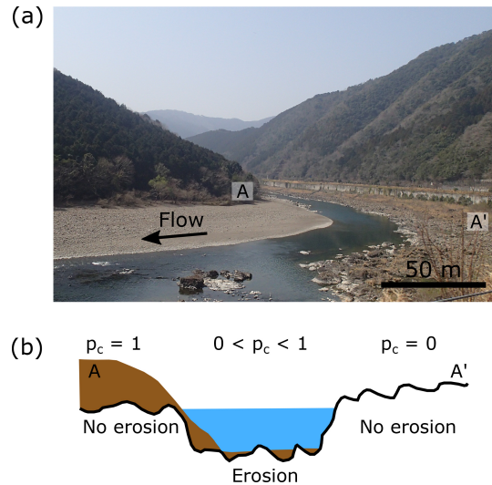
Figure 17. (a) Image of a reach of the Shimanto River, Shikoku, Japan, showing partial cover with alluvium. (b) Sketch of cross section A–A’ (with strong vertical exaggeration) indicating inferred regions of erosion and no erosion.
