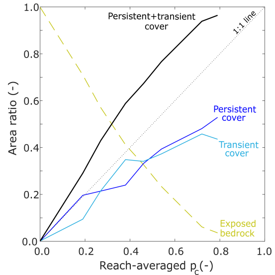
Figure 10. Reach-averaged area ratios of persistently exposed bedrock, transient alluvial cover, persistent alluvial cover, and persistent + transient alluvial cover as a function of reach-averaged areal cover fraction.
