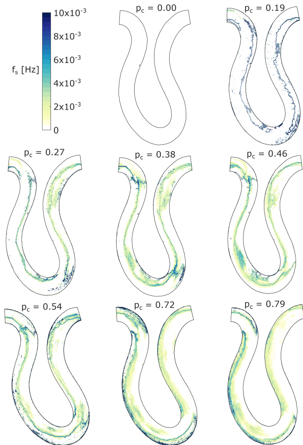
Figure 15. Maps of the frequency of strikes for all experimental conditions. The frequency shown is based on the number of images. Dividing the values by 10 s, which is the time between images, will give the actual frequency (Hz).
