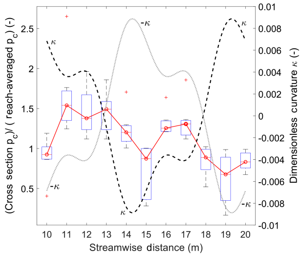
Figure 13. Box plots of the normalized cross-sectionally averaged areal fraction of alluvial cover in the middle bend of the Kinoshita flume. The dimensionless curvature of the flume \kappa and its negative value -\kappa are plotted to better show the salient trends.
