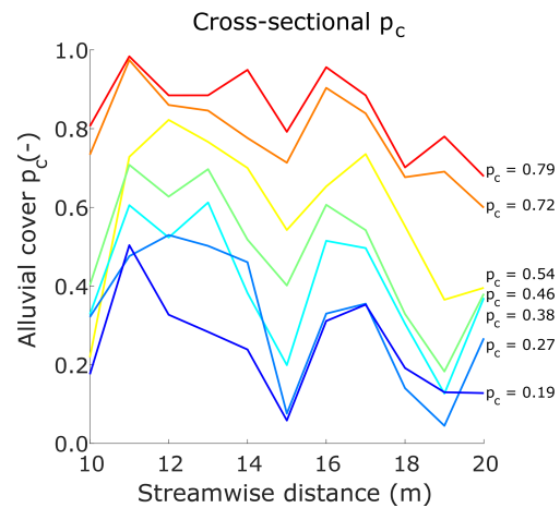
Figure 11. Cross-sectional averages of the areal fraction of alluvial cover for all experimental runs. Local values were extracted every meter between streamwise locations 10 and 20 m. The legend indicates the corresponding reach-averaged values.
