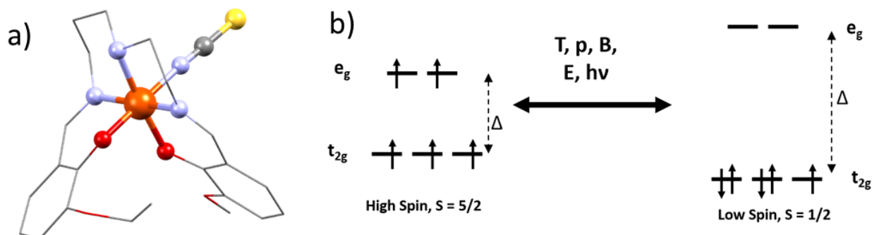
Figure 1 a) Molecular structure of the [Fe(L)NCS] complex. Fe-orange, N-blue, O-red, C-grey, S-yellow. b) Resulting energy levels for the HS and LS states split by energy \Delta .
