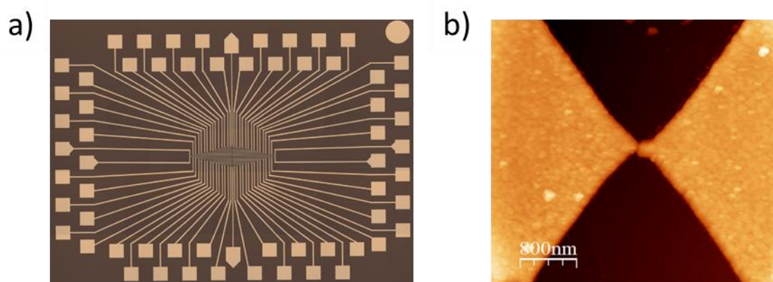
Figure 2 a) Device containing 15 nanojunctions with bonding pads. b) Nanogap after feedback controlled electromigration.
