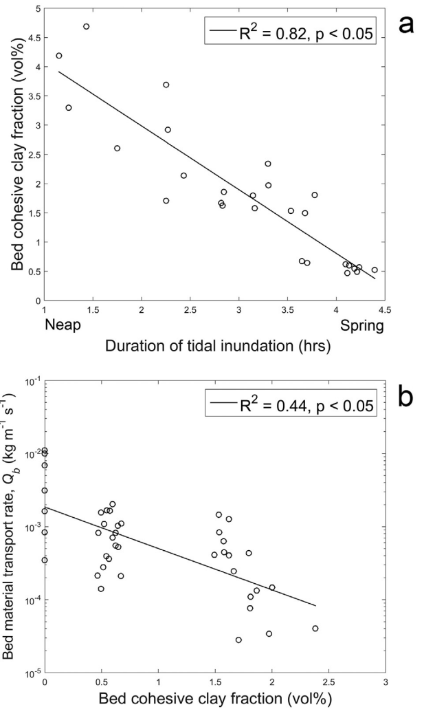
Fig. 10. (a) Relationship between duration of tidal inundation, in hours, and bed cohesive clay content for each tidal inundation period ( n = 27 ). (b) Relationship between bed material transport rate and bed cohesive clay fraction (maximum flood and ebb values for each tidal inundation period, n = 41 ). The data for clay-free sand ( D_{50} = 238 \mu\text{m} ) from Baas et al. (2000) are also included for zero cohesive clay values.
