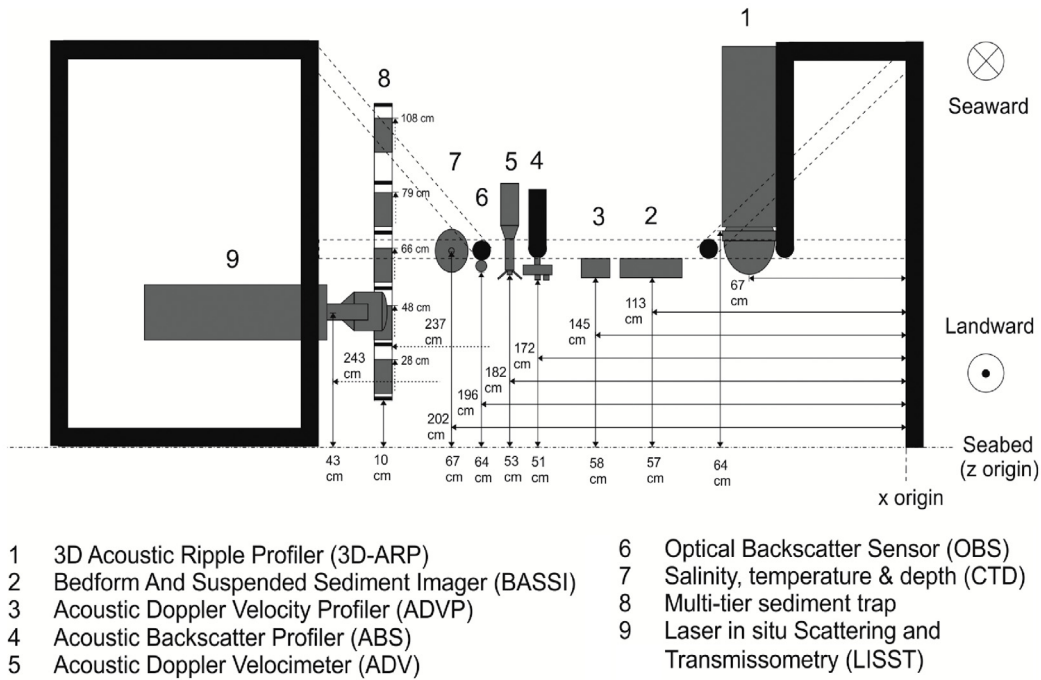
Fig. 3. Instrument frame SEDbed at Site 2, looking seaward towards Little Hilbre and Hilbre Island (top), and diagram of instruments on frame (bottom). Initial heights above the sediment bed are shown, with horizontal distance relative to the edge of the frame.
