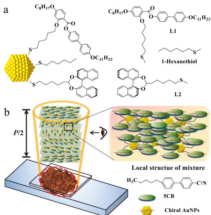
Chart 1. (a) Sketch of a segment of functionalized gold nanoparticle ChirAuLC , (b) Cartoon introducing the concept of induced chiral structure in host 5CB by the macro-chiral liquid crystal nanoparticles ( ChirAuLC ).
