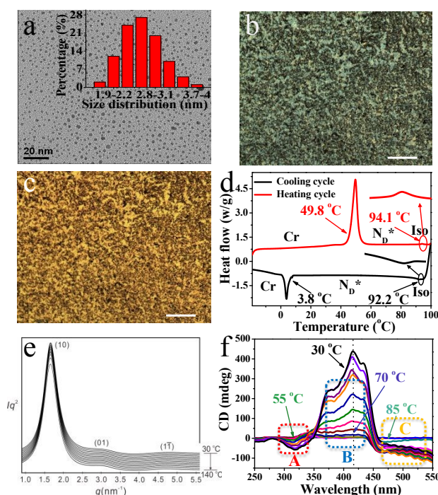
Fig. 1 (a) TEM image of 2.5 nm AuDLC* nanocomposite (insert: the size distribution of AuDLC*). POM micrographs of AuDLC* (b) 86.5 °C (90° crossed polarizer) ( \times 100 \mu\text{m} ). (c) 37.8 °C (90° crossed polarizer) ( \times 100 \mu\text{m} ). (d) DSC of AuDLC* at heating and cooling rate of 10.0 °C/min. (e) SAXS diffractograms of AuDLC* on heating from 30 °C to 140 °C. (f) SRCD spectra of sheared AuDLC*. Recorded in 5 °C steps on cooling from 100 °C to 30 °C. The enlarged plots in dotted regions A-C are shown in Fig. S12b-d. The CD intensities at a selected wavelengths in each region (A, B and C) are plotted as a function of temperature in Fig. S13 and these plots clearly show the difference in the formation process between the two helical structures.
