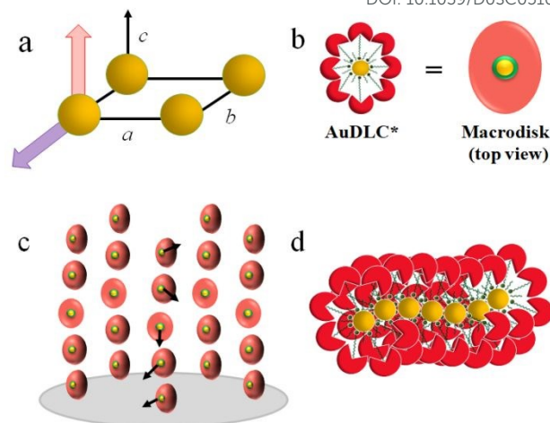
Fig. 2 Schematic representation of (a) p2 lattice with parameters a = 4.17 nm, b = 2.52 nm and the angle \gamma \sim 48.4^\circ ; spatial direction c not defined by the lattice. Red arrow: N D * helix axis; Purple arrow: plasmonic interactions. (b) AuDLC* macrodisk. Yellow: gold core; Red: PA unit; Green: chiral sheath. (c) N D * phase formed by functionalized NPs. (d) Chiral assembly behaviour of gold NPs along the axis of smallest lattice parameter b .
