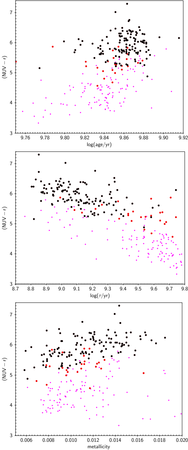
Figure 13. Distribution of rest-frame (\text{NUV}-r) colour for the three red sequence subsamples (coloured as previously) as a function of (top) stellar population age, (middle) star formation timescale \tau , and (bottom) metallicity.
