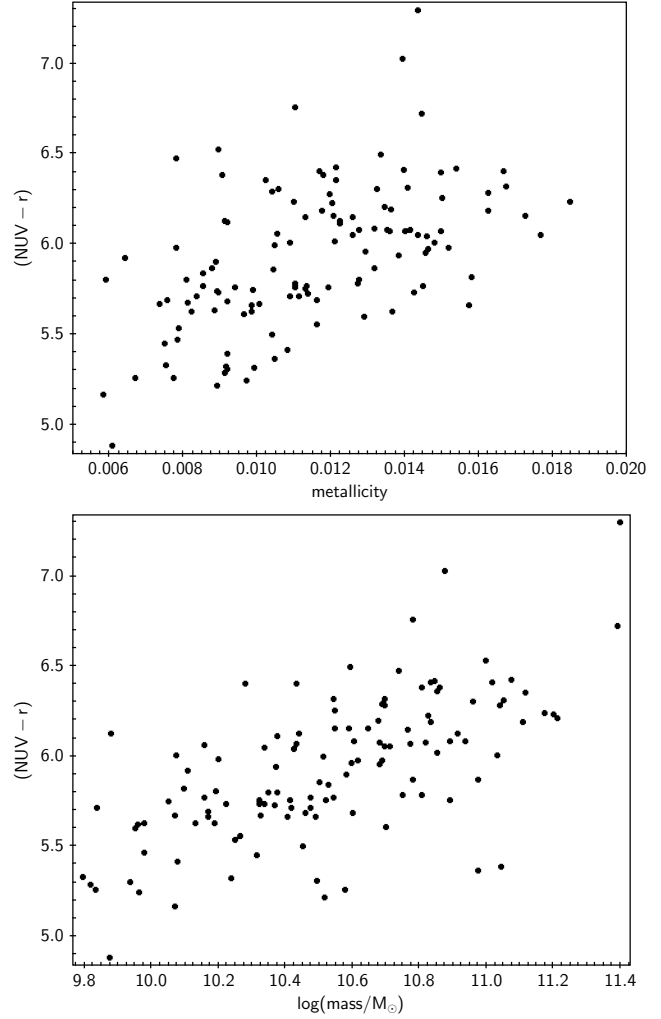
Figure 14. Distribution of rest-frame (\text{NUV}-r) colour as a function of stellar metallicity as in the bottom panel of Figure 11, but for the final NUV+WISE red sequence only (top panel), and as a function of stellar mass for the same sample (bottom panel).
