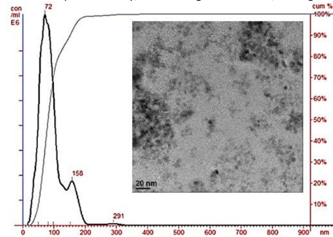
Fig 2: Nanoparticle tracking analysis of the prepared coated NPs with the silica CB-cyclam-Ni coating suspended in deionised water; the TEM image is inset.
