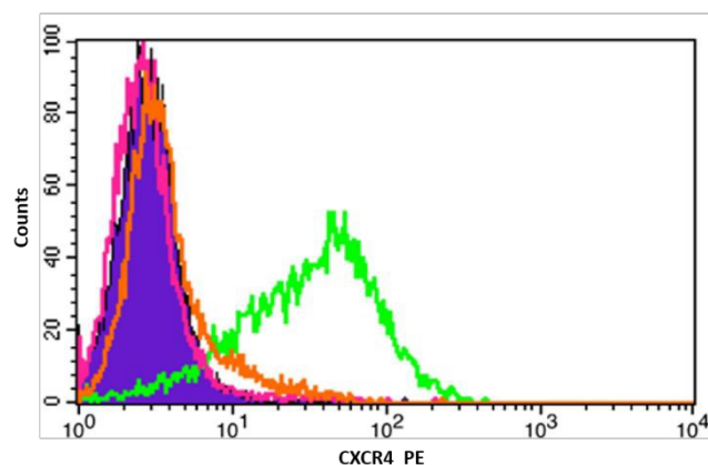
Figure 3: Flow cytometry histogram of the binding of anti-CXCR4-PE (12G5) on the cell surface of Jurkat cells. Negative (solid purple), Anti-CXCR4-PE mAb only (green), and competition with NPs (pink & orange).
