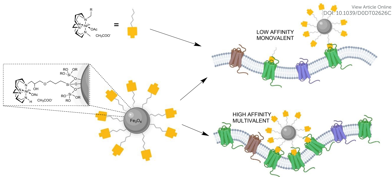
Figure 1: A low affinity mono-macrocycle binding unit can be used to generate high affinity CXCR4 chemokine receptor (represented as the green GPCR in the cell membrane) binding nanoparticles through multivalent receptor binding interactions. The approach could be used to optimise affinity for high CXCR4 expressing tissues and cells.
