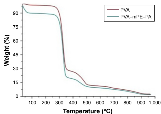
Figure 6 TGA of PVA membrane and PVA/mPE/PA nanocomposites.
