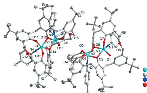
Fig. 3 Molecular structure of \{[\text{V}(\text{Np}-\text{CH}_3\text{C}_6\text{H}_4)]_2\text{L}^1\} ( 3 \cdot 7\text{MeCN} \cdot 0.5\text{CH}_2\text{Cl}_2 ). (H atoms and \text{CH}_2\text{Cl}_2 molecules are omitted for clarity).
