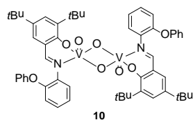
Scheme 1. Mono-vanadium complexes screened in this study
