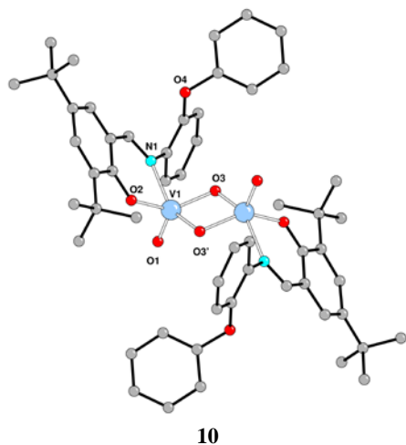
Figure 2. CAMERON representation of the dinuclear \mu -oxo complex 10 showing the atom numbering scheme. Hydrogen atoms and solvent (MeCN) molecules have been omitted for clarity.
