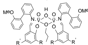
R = Ad; R' = Me (11); R = C(Me) 2 Ph; R' = Me (12); R = tBu; R' = H (13)
