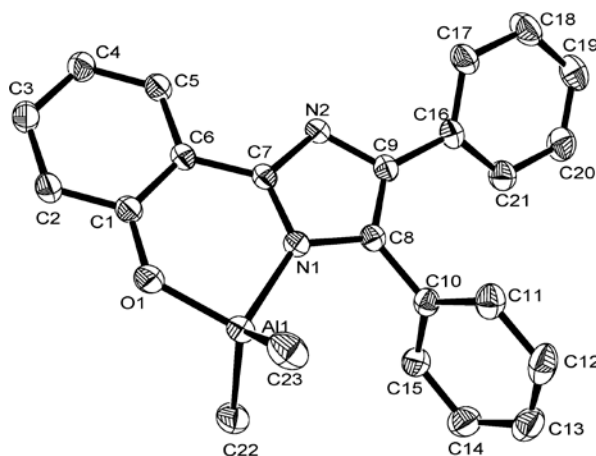
Figure 3. ORTEP drawing of C4 with thermal ellipsoids drawn at the 30 % probability level. Hydrogen atoms are omitted for clarity.
