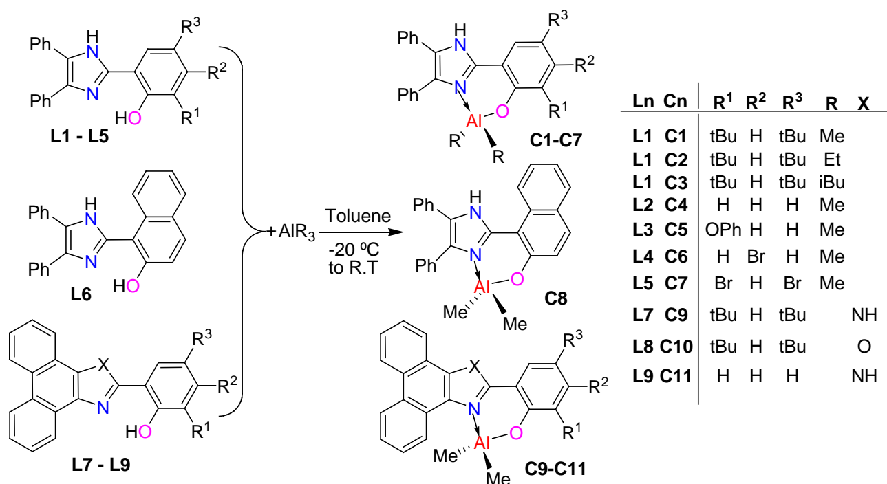
Scheme 1 Synthesis of the dialkylaluminum complexes C1–C11
