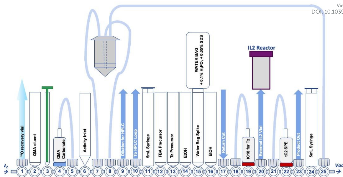
Figure 2. A schematic representation of the GE FASTLab™ cassette developed for the automated radiosynthesis of [^{18}\text{F}]\text{TTCO-IL2} ; a detailed description of the cassette setup appears in the supporting information (ESI Figure S14).
