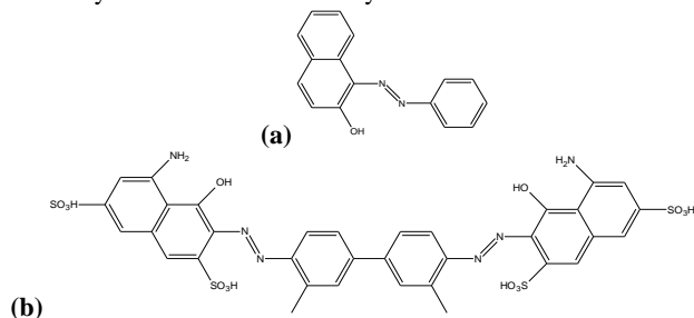
Figure 3. Chemical structures of (a) hydrophobic Sudan I, and (b) hydrophilic Trypan Blue.
