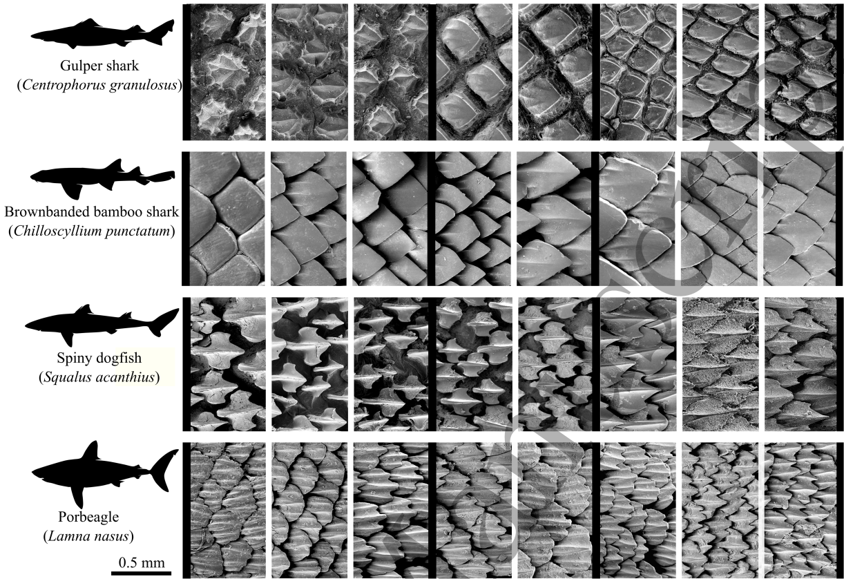
Figure 1. Scanning Electron Microscope (SEM) images of shark skin denticles taken from the flank along a central line from head to tail (left to right). Denticles are oriented such that the flow direction is approximately from left to right. Note the riblet features protruding from the denticles of the Squalus acanthius and Lamna nasus species. Image adapted from Fletcher (2015).
