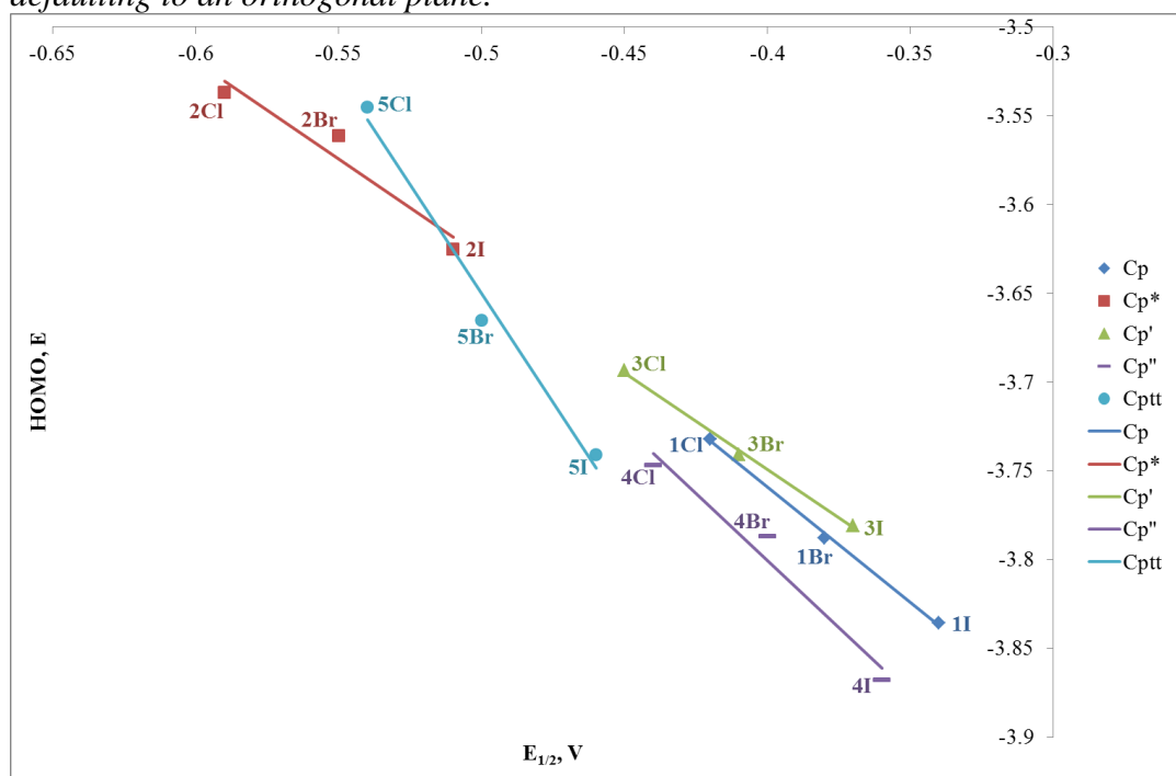
Figure 9: Frontier Kohn Sham molecular orbitals of 1Cl : (a) HOMO, (b) HOMO-1, (c) HOMO-2. The models were orientated such that the Fe-X vector corresponded to the z -axis and the Fe-Ct was selected as the basis for the x -axis, with the y -axes defaulting to an orthogonal plane.
