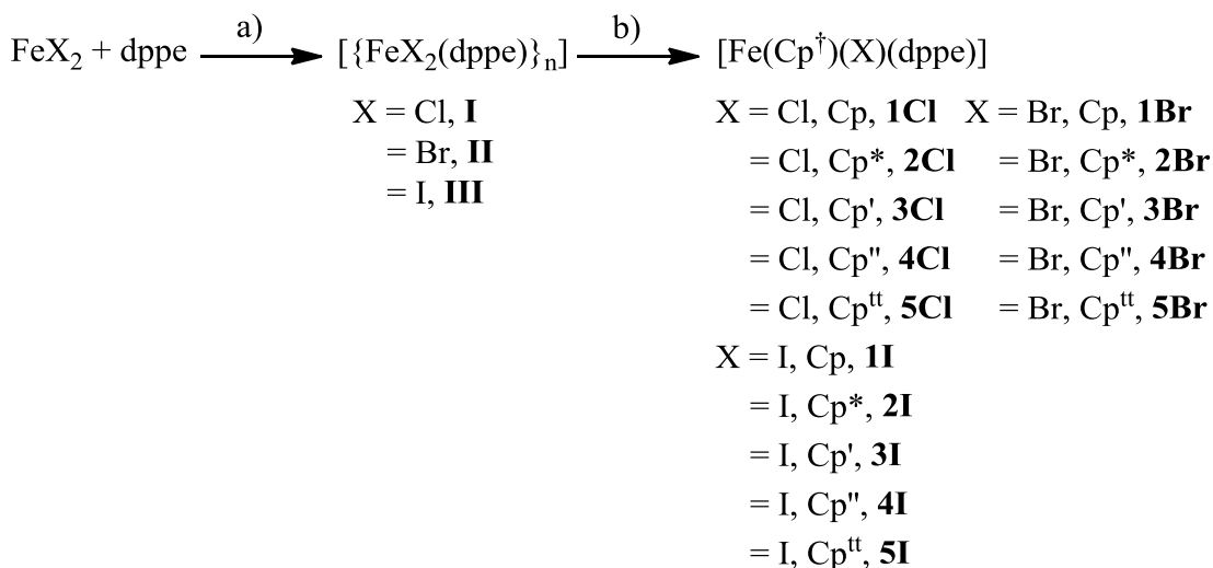
Scheme 1: Synthesis of I , II , III , 1Cl-5Cl , 1Br-5Br , 1I-5I . Reagents and conditions: a) THF, \Delta ; b) LiCp/NaCp/KCp † , toluene, -78 °C, -LiCl/KCl/NaI/KCl/KBr/KI.
