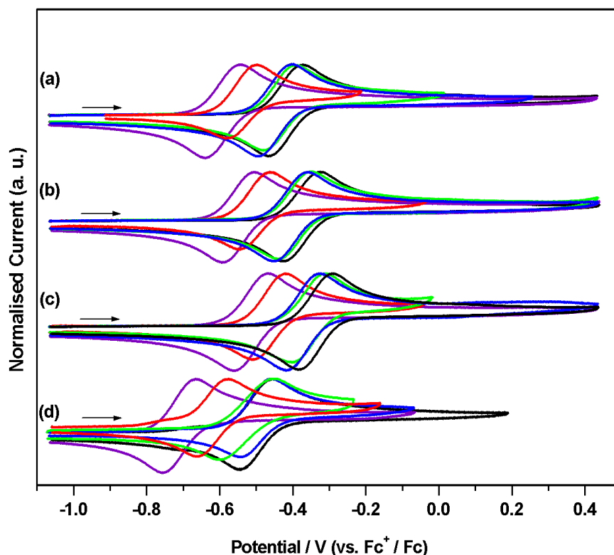
Figure 7: Cyclic voltammograms showing OX for (a) [Fe(Cp † )(Cl)(dppe)], (b) [Fe(Cp † )(Br)(dppe)], (c) [Fe(Cp † )(I)(dppe)] and (d) [Fe(Cp † )(H)(dppe)] (Cp † = Cp (black), Cp* (violet), Cp' (blue), Cp'' (green), Cp tt (red)). In THF containing [ n Bu 4 N][BF 4 ] (0.5 M) as supporting electrolyte, at 0.1 Vs -1 (except 4H , at 1 Vs -1 ). Currents are normalised to I p a for clarity. Typical currents obtained from CV
