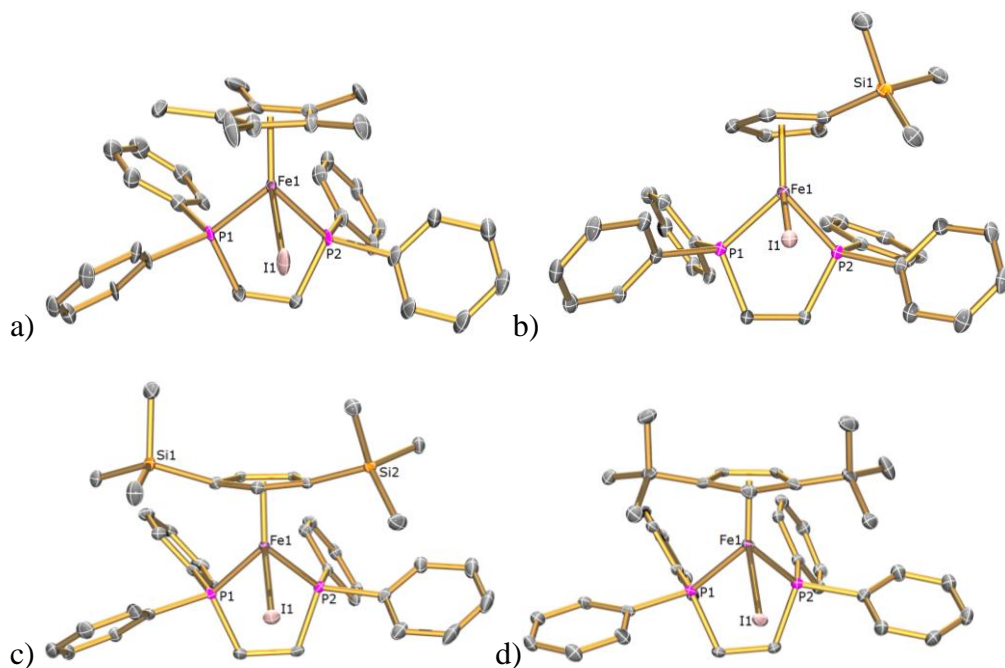
Figure 4: Solid state structures of a) 2I , b) 3I , c) 4I , d) 5I with ellipsoids set at 40 % probability. Hydrogen atoms are omitted for clarity.
