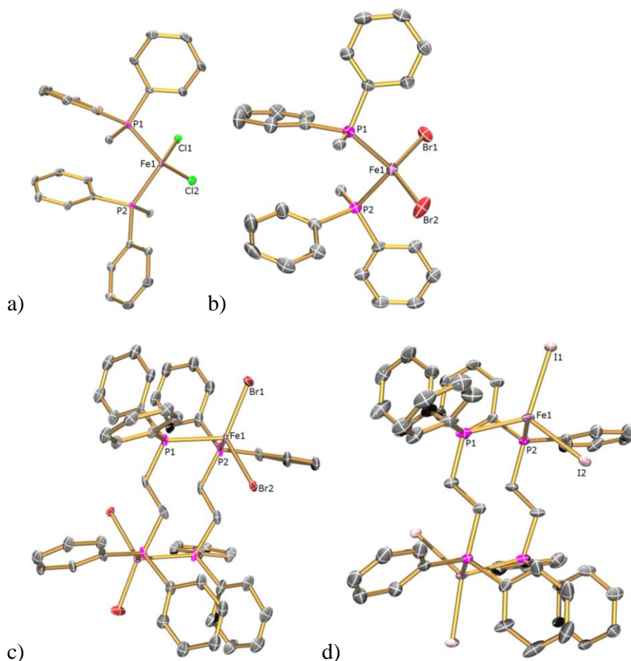
Figure 1: Solid state asymmetric unit structures of a) I (polymer), b) II (polymer), c) IIa (dimer), d) III (dimer) with ellipsoids set at 40 % probability. Hydrogen atoms and minor disorder components are omitted for clarity. Selected bond lengths (Å) and angles (°): a) Fe1–Cl1 2.2416(16), Fe1–Cl2 2.2403(15), Fe1–P1 2.4422(16), Fe1–P2 2.4849(16), Cl1–Fe1–Cl2 127.14(6), Cl1–Fe1–P1 104.65(6), Cl1–Fe1–P2 100.74(6), Cl2–Fe1–P1 100.80(6), Cl2–Fe1–P2 111.50(6), P1–Fe1–P2 111.80(5); b) Fe1–Br1 2.368(8), Fe1–Br2 2.370(9), Fe1–P1 2.468(12), Fe1–P2 2.454(13), Br1–Fe1–Br2 121.22(3), Br1–Fe1–P1 100.24(4), Br1–Fe1–P2 114.25(4), Br2–Fe1–P1 108.10(4), Br2–Fe1–P2 105.65(4), P1–Fe1–P2 107.54(4); c) Fe1–Br1 2.375(2), Fe1–Br2 2.372(2),
