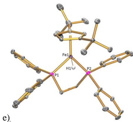
Figure 6: Solid state structures of a) 1H , b) 2H , c) 3H , d) 4H , e) 5H with ellipsoids set at 40 % probability. All hydrogen atoms except those for the hydride atoms are omitted for clarity.
