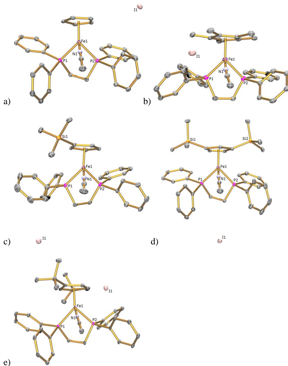
Figure 5: Solid state structures of a) 1SIP , b) 2SIP , c) 3SIP , d) 4SIP , e) 5SIP with ellipsoids set at 40 % probability. Hydrogen atoms are omitted for clarity.
