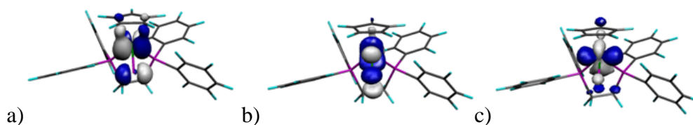
Figure 9: Frontier Kohn Sham molecular orbitals of 1Cl : (a) HOMO, (b) HOMO-1, (c) HOMO-2. The models were orientated such that the Fe-X vector corresponded to the z -axis and the Fe-Ct was selected as the basis for the x -axis, with the y -axes defaulting to an orthogonal plane.
