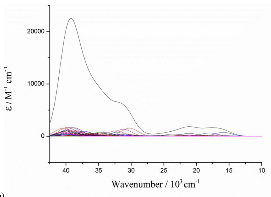
Figure 8: a) UV-vis spectra of 2Cl at 1.25 mM and 0.0125 mM (insert) in THF solution. b) Predicted UV-vis spectrum of 2Cl showing the individual electronic transitions and the combined total in the gas phase.
