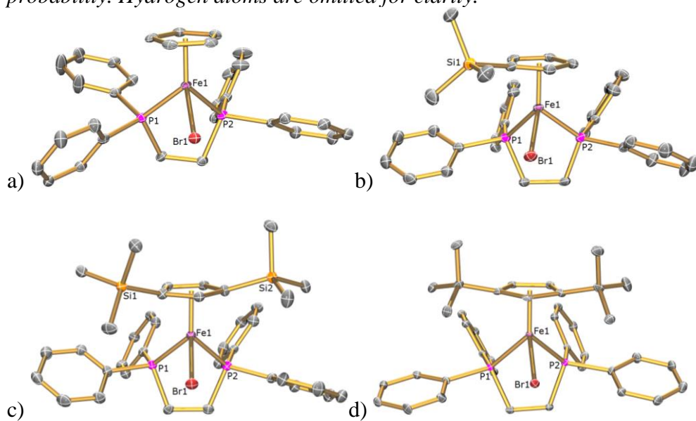
Figure 3: Solid state structures of a) 1Br , b) 3Br , c) 4Br , d) 5Br with ellipsoids set at 40 % probability. Hydrogen atoms are omitted for clarity.
