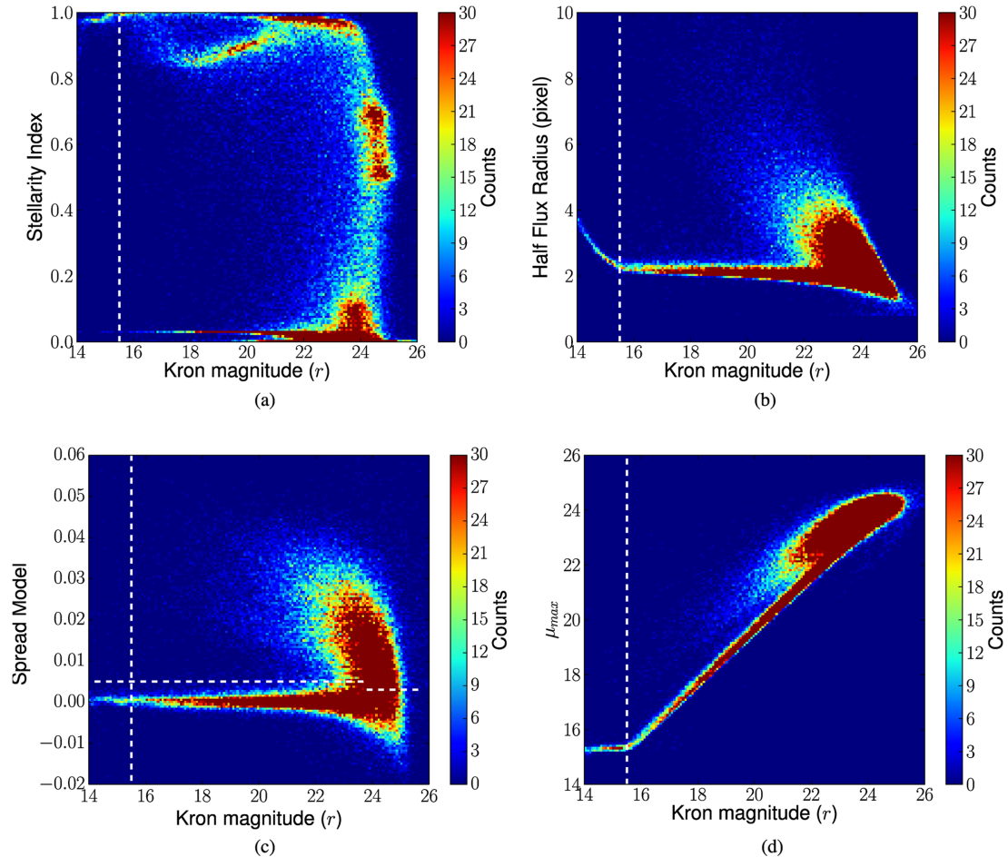
Figure 8. Two-dimensional histogram of SECTOR stellerity index (panel a), half-light radius (panel b), spread model (panel c), and \mu_{\max} (panel d) as a function of Kron magnitude for sources in r -band image of field 12. The vertical dashed line in all panels is the magnitude limit adopted for saturated objects. The horizontal lines in panel (c) mark the limit used to separate stars and galaxies (see text). The points are colour coded according to their number counts as reported in the vertical colour bars.
