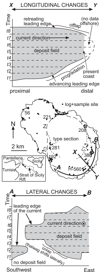
Figure 3. Time ( t_1 – t_8 ) versus distance plots for Green Tuff (Pantelleria, Italy) in longitudinal (X–Y) and circumferential (A–B; current coming out of page) sections, showing that base and top of deposit are diachronous, with onlap and offlap recording how current waxed ( t_1 – t_4 ) and then waned ( t_5 – t_8 ). Location map (center) shows distribution of data points and sections, and spot heights of topographic highs (in meters). In the south, current flow path shifted laterally as current waxed, recorded as lateral overlap from east to west ( t_5 – t_7 ). As current waned, it shifted eastward again ( t_5 – t_7 ) until only narrow finger of current persisted ( t_8 ). Widespread preservation of original top surface of ignimbrite means that offlap relations are not just an artifact of subsequent erosion.
