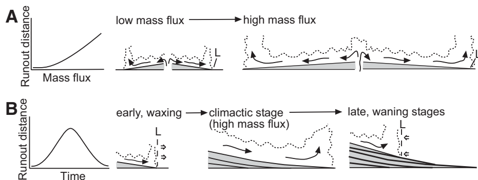
Figure 4. Eruptive mass flux versus current runout distance (from Bursik and Woods, 1996). A: Radial, sustained density current at low mass flux travels short distance before lift-off point (L), where current lofts following density loss by deposition and mixing dilution during transport (depletive flow). At higher mass fluxes, current travels further from source. B: Emplacement of Green Tuff density current reconstructed: leading edge advances during initial stages of waxing mass flux, to climax (when runout distance peaks), followed by leading edge retreat during waning stages. Resultant deposit (gray; black lines are entrachrons) has diachronous base and top and records current evolution with time and space.
