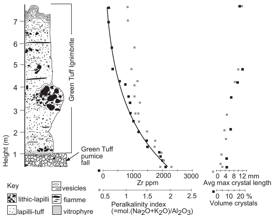
Figure 1. Vertical section of Green Tuff ignimbrite (Pantelleria, Italy), showing gradational compositional and mineralogical variations, with gradational variations in Zr values with height; 80 vertical sections logged for the study show similar variations. Deposit is mostly massive with well-preserved clastic textures. Upper parts typically show rheomorphic deformation.
