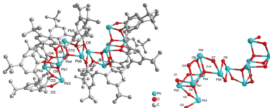
Fig. 7 Molecular structure and core of [\text{Pb}_{12}(\text{L}^8)_2\text{O}_4]\cdot 12\text{MeCN} ( 7\cdot 12\text{MeCN} ). For clarity, hydrogen atoms and solvent molecules are not shown. Selected bond lengths (Å) and angles (°): Pb(4)–O(10) 2.356(6), Pb(4)–O(9) 2.335(6), Pb(4)–O(5) 2.278(6), Pb(4)–O(4) 2.370(6), Pb(2)–O(9) 2.247(6), Pb(2)–O(3)–O(2) 2.454(7), Pb(2)–O(4) 2.287(6), Pb(2)–O(1) 2.388(7), Pb(6)–O(6) 2.664(7), Pb(1)–O(10) 2.281(6), Pb(1)–O(9) 2.374(7), Pb(1)–O(8) 2.419(7), Pb(5)–O(10) 2.275(6), Pb(5)–O(5) 2.421(6), Pb(3)–O(9) 2.269(7), Pb(3)–O(2) 2.192(7), O(10)–Pb(4)–O(4) 119.7(2), O(9)–Pb(4)–O(10) 74.4(2), O(9)–Pb(4)–O(4) 72.3(2), O(5)–Pb(4)–O(10) 70.0(2), O(5)–Pb(4)–O(9) 111.7(2), O(9)–Pb(2)–O(3) 71.1(2), O(9)–Pb(2)–O(4) 75.5(2), O(4)–Pb(2)–O(3) 80.8(2), O(10)–Pb(1)–O(9) 75.1(2).
