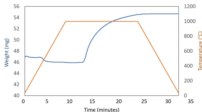
Figure 3. TGA curve showing an increase in the weight of the sample \text{Sr}_2\text{CuO}_3 as \text{CO}_2 is introduced at 1000^\circ\text{C} forming \text{Sr}_2\text{CuO}_2(\text{CO}_3) .
