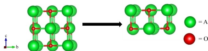
Figure 2. The crystal structure of an AO compound ( A = \text{Ca} , \text{Sr} and \text{Ba} ) is on the left, with the reduced cluster on the right.
