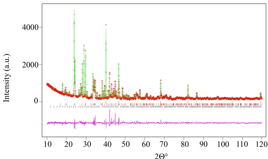
Figure 9. Rietveld refinement pattern of \text{Ba}_2\text{PdO}_3 after reacting with \text{CO}_2 , showing the observed (red crosses), calculated (green) and difference (purple) patterns. The ticks represent \text{Ba}_{11}\text{Pd}_{11}\text{O}_{20}(\text{CO}_3)_2 (black), \text{BaCO}_3 (red) and Pd metal (blue).
