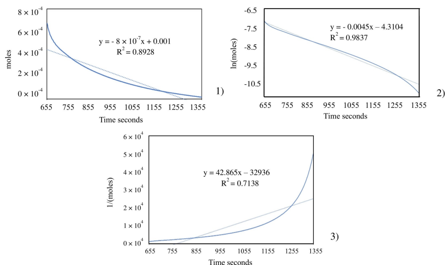
Figure 7. Three concentrations vs. time graphs, (1) moles of \text{Sr}_2\text{CuO}_3 vs. time seconds, (2) \ln(\text{moles}) of \text{Sr}_2\text{CuO}_3 vs. time seconds, and (3) 1/(\text{moles}) of \text{Sr}_2\text{CuO}_3 vs. time second. Equations of trendlines and R^2 are given for each graph. The best fit ( R^2=0.9837 ) is obtained for a first-order kinetics.
