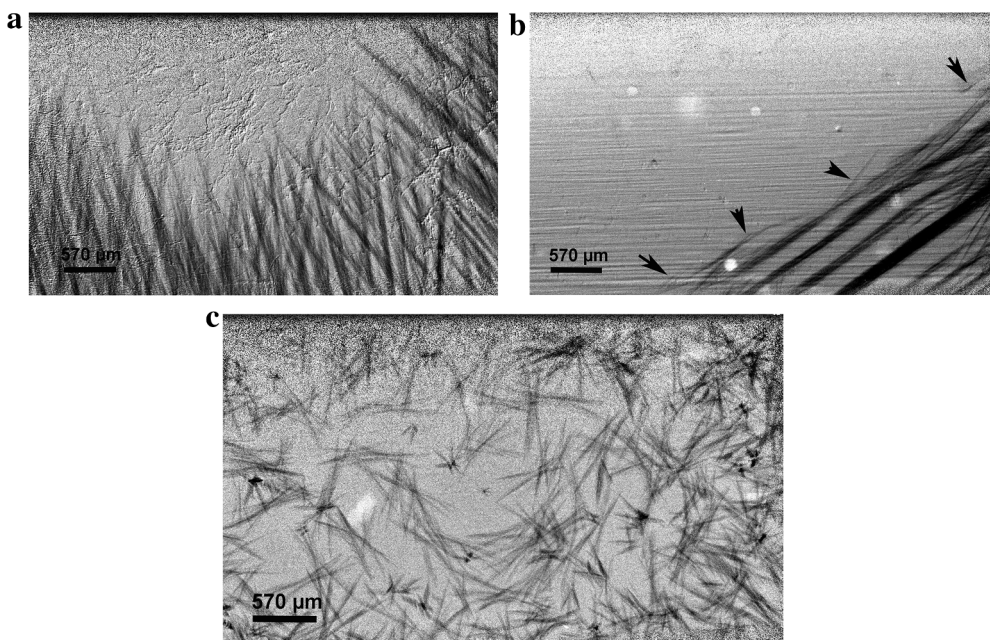
Fig. 14. Fragmentation of Al 2 Cu dendrites in and Al-35 wt% Cu alloy ( in situ synchrotron X-ray study): (a) elongated dendrites growing without USP; (b) fragmentation (shown by arrows) of dendrites by acoustic streaming (ultrasonic source is above the left top corner); and (c) refined equiaxed crystals formed after the end of USP.
