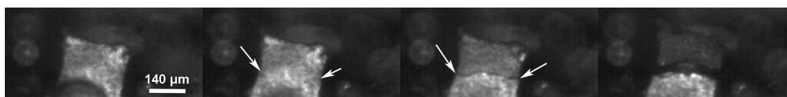
Fig. 13. Images of a primary \text{Al}_3\text{Ti} crystal fragmented by a pulsating bubble (seen on the first frame). Arrows show the fatigue crack initiation and propagation. The field of view is 337.28 \times 739.65\mu\text{m}^2 and the images were recorded at 10^5 fps [50].
