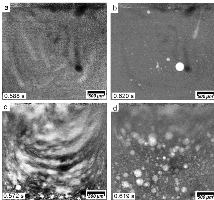
Fig. 7. Synchrotron X-ray observation of flow patterns and cavitation bubble population in an Al–10 wt% Cu alloy (a, b) and an Al–10 wt% Cu alloy with 0.05 wt% of 80-nm Al 2 O 3 particles (c, d) (700 °C, 30 kHz, 800 W/cm 2 ) [38]. (a, c)–during USP, (b, d)–immediately after USP has been stopped.
