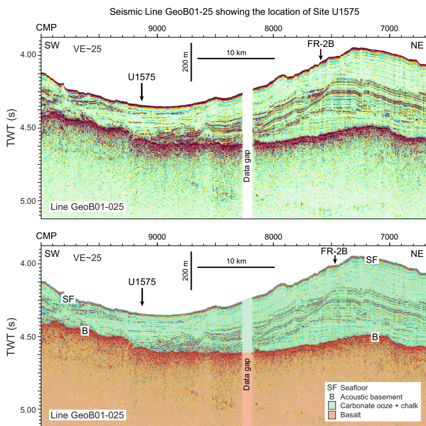
Figure F12. Seismic Line GeoB01-25. Top: seismic profile. Arrows show locations of Site U1575 and proposed Site FR-2B. Bottom: seismic line interpretation. TWT = two-way travelttime, VE = vertical exaggeration.
