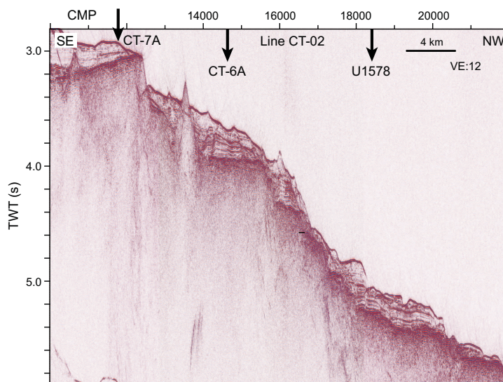
Figure F27. Section of Seismic Line TN373-CT2B showing the northwest flank of the Center track guyot. Arrows = locations of Site U1578 and proposed alternate Sites CT-6A and CT-7A. VE = vertical exaggeration.
