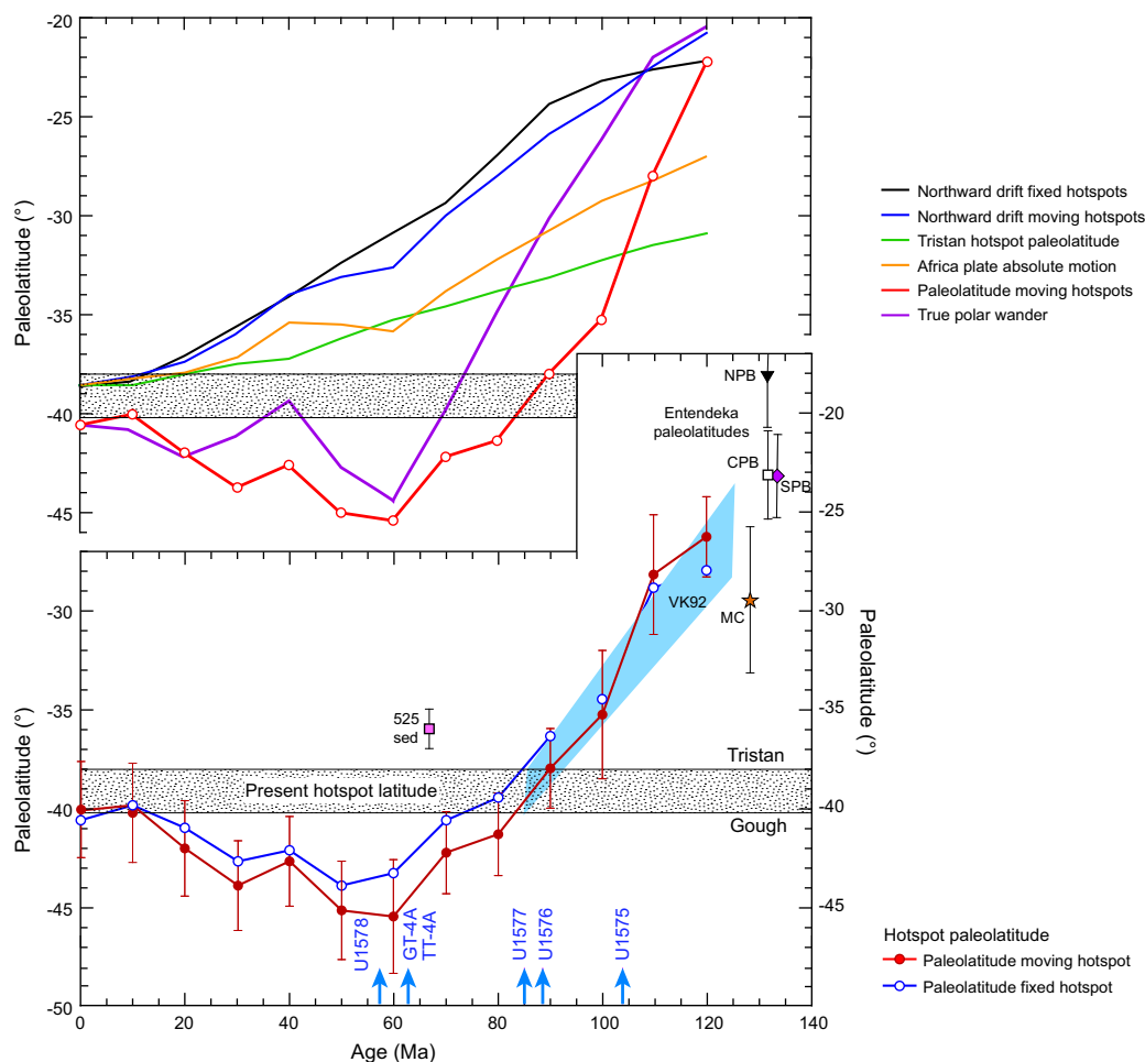
Figure F7. Predicted paleolatitude drift of the TGW hotspot, hotspot models, and TPW. Bottom: paleolatitude estimates. Red line with dots = estimated paleolatitudes calculated from the global average African plate apparent polar wander path (Torsvik et al., 2008) based on a plate motion model with moving hotspots (Doubravine et al., 2012). Thin vertical lines = 95% confidence limits based on paleomagnetic data scatter only. This polar wander path was constructed with a 20 My window length, averaged every 10 Ma. Blue line with dots = the same paleolatitude curve for a fixed hotspot model (Torsvik et al., 2008). Pink square = a paleolatitude determined for 60–75 Ma sediments from Site 525 (Chave, 1984). Its departure from the paleolatitude curve may be a result of inclination shallowing that is common for sediments (Verosub, 1977). Black triangle (NPB), white square (CPB), and purple diamond (SPB) = paleolatitudes from the north, central, and south Parana flood basalts, respectively (Ernesto et al., 1990, 1999). Orange star (MC) = paleolatitude of Messum gabbros in the Etendeka province (Renne et al., 2002). Blue band (VK92) = hotspot drift estimated by Van Fossen and Kent (1992). Blue arrows = estimated ages of proposed drill sites from an age progression model (Homrighausen et al., 2019, 2020). Top: northward drift and TPW. Red line with circles = paleolatitudes estimated from paleomagnetic data (same as lower plot). Black line = the northward drift of a seamount with time if formed at the Tristan hotspot location (Schlömer et al., 2017), assuming a fixed hotspot model (Torsvik et al., 2008). Blue line = a moving hotspot model (Doubravine et al., 2012). Green line = the paleolatitudes of the Tristan hotspot from a mantle flow model (Doubravine et al., 2012), indicating ~7° southward motion in 120 Ma. Orange line = the northward drift of the African plate in the moving hotspot model (Doubravine et al., 2012). It is less than the fixed hotspot model because the Tristan hotspot is modeled as moving south. Adding the hotspot motion to the moving hotspot model absolute motion equals the total northward motion indicated by the morphology of the TGW chain and the fixed hotspot model. All absolute motion models indicate that the African plate moved nearly monotonically northward, so they do not explain the rapid southward shift in paleolatitudes during the Late Cretaceous or the northward offset of paleolatitudes during the early Cenozoic. The difference between modeled and observed paleolatitudes implies significant TPW (purple curve) (Doubravine et al., 2012).
