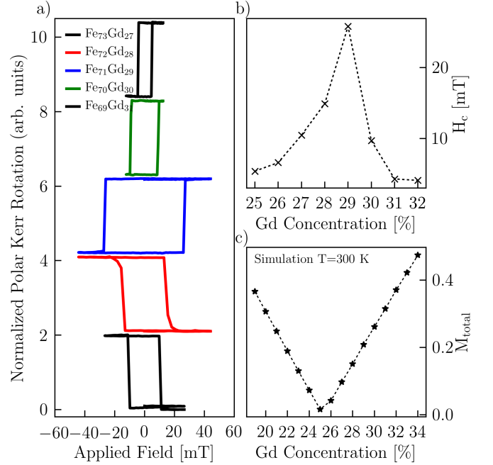
FIG. 1. a) Magnetic hysteresis of different FeGd-alloys between 27-31 % Gadolinium probed by the magneto optical Kerr rotation at 300 K. The use of an objective lens that is close to the electromagnet's gap induces an additional slope on the Kerr hysteresis data, due to a Faraday effect in the lenses' glass. This slope, which is independent of the sample, was numerically removed from this figure. The polarity of the hysteresis changes as the system crosses the compensation. The coercivity diverges as the Gd-concentration approach the compensation point. b) The experimentally measured coercive field H_c of subfigure a) as function of the Gd concentration. The line is guidance to the eye. c) The simulated total magnetization of the FeGd-alloy at 300 K as function of the Gd concentration. The simulated magnetization compensation temperature is slightly lower (between 25 % -26 %) than the experimental one with the drawn line being guidance to the eye.
