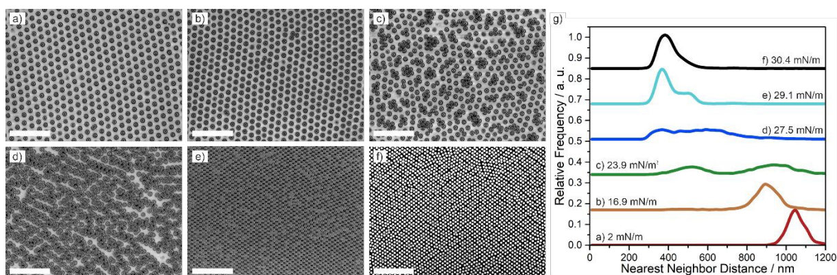
Figure 4: Interfacial phase behavior of 295 nm-5 mol% core-shell particles. a-f) SEM images taken after deposition to a solid substrate from the air/water interface at different surface pressures. g) Corresponding nearest neighbor distributions. The particles undergo a phase transition from hexagonal non-close packed arrangements (a,b) to a rhomboid lattice (e) and
