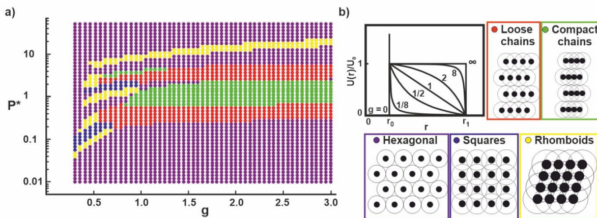
Figure 7: Calculated phase diagram of core-shell particles interacting via Jagla potentials with a shell to core ratio r_1/r_0 of 3. a) Calculated phase diagram for different g parameters and external pressures. The different colors correspond to different phases: hexagonal arrangements are colored violet, loose chains are red, compact chains green, squares blue and rhomboids yellow. b) Interaction potential used for the calculations according to Jagla and snapshots of the calculated minimum energy phases.
