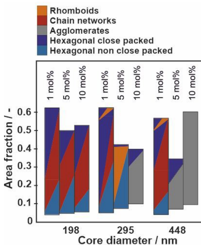
Figure 6: Overview of the interfacial phase behavior of all synthesized core-shell particles with different core diameter and crosslinking density upon compression at the air/water interfaces. The bars color-code the existence and coexistence of phases of the particle systems at different stages of compression (i.e. at different area fractions). Individual phases are represented by different colors; more than one color in the horizontal profile of a bar represents a coexistence of the phases at the corresponding area fraction.
