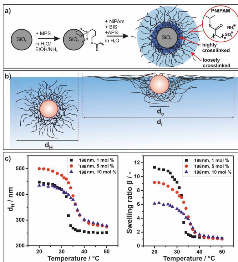
Figure 1: Synthesis and structure of PNIPAM-SiO 2 core-shell particles. a) Schematic illustration of the core-shell particle synthesis and architecture. b) Schematic illustration of the core-shell particles in bulk and adsorbed to the air/water interface with the relevant dimensions given by the particle core diameter d_c , the hydrodynamic diameter d_H in bulk and the diameter of the particle and its extended corona at an air-water interface d_i . c) Representative temperature-dependent
