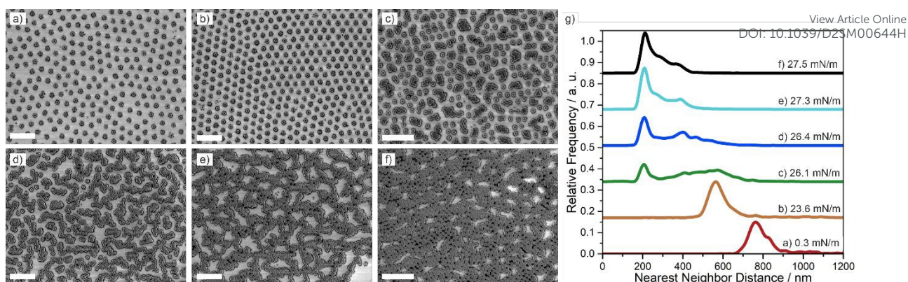
Figure 3: Interfacial phase behavior of 198 nm-10 mol% core-shell particles. a-f) SEM images taken after deposition to a solid substrate from the air/water interface at different surface pressures. g) Corresponding nearest neighbor distributions. The particles undergo a phase transition from hexagonal non-close packed arrangements (a,b) to chain-like networks (d-e) to a dense chain network (f) upon compression. Scale bar: 2 \mu\text{m} .
