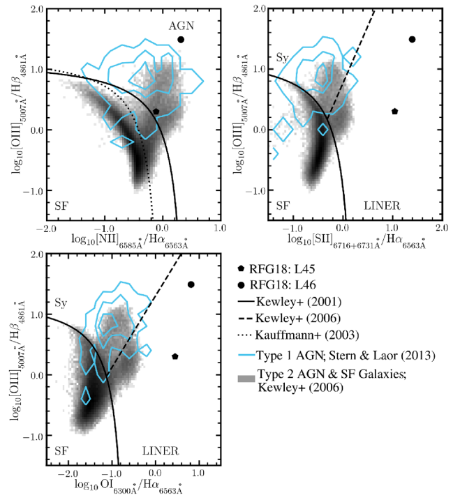
Figure 9. BPT diagrams from our simulations (black symbols), star-forming galaxies, and type 2 AGN from SDSS (Kewley et al. 2006; grey 2D histogram), and type 1 AGN from SDSS with bolometric luminosities > 10^{45} \text{ erg s}^{-1} (Stern & Laor 2013; blue contours). The black solid and dotted curves show the boundaries between star-forming and active galaxies from Kewley et al. (2001) and Kauffmann et al. (2003), respectively, while the black dashed lines show the boundary between LINERs and Seyferts from Kewley et al. (2006). The [\text{S II}]_{6716+6731\text{Å}} / \text{H}\alpha_{6563\text{Å}} and [\text{O I}]_{6300\text{Å}} / \text{H}\alpha_{6563\text{Å}} line ratios are up to an order of magnitude higher in the simulations than is seen in the observations, due to strong X-ray heating in the assumed partially-obscured incident quasar spectrum and unresolved ionized layers.
