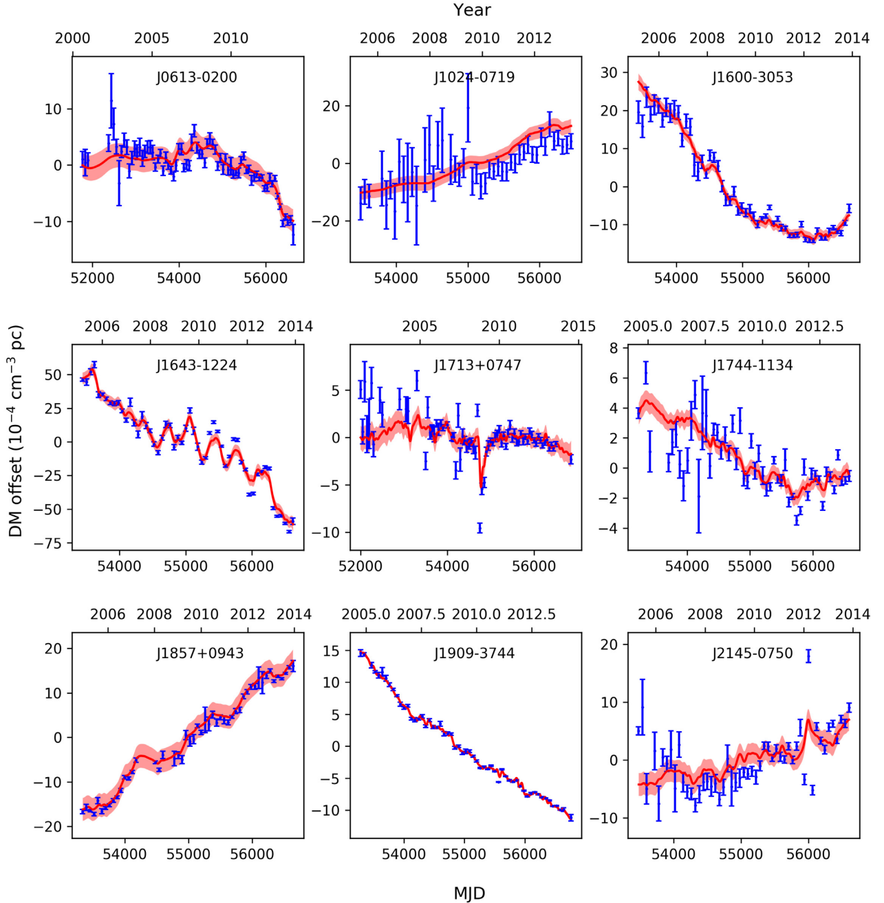
Figure 3. The time-dependent DM variations for pulsars that are observed by all three PTAs obtained using the DMMODEL (blue) as described in VersionA (see Section 4.1). Note that the mean DM is subtracted and only the variation is plotted. For comparison, the DM variations obtained using the power-law model described in VersionB (see Section 4.2) are overplotted (red), and their uncertainties are estimated using a Gaussian process regression method. The overall features in DM variations obtained from the two versions are consistent with each other within their measured uncertainties. Note that we omitted PSR J1939+2134 in this figure because of its complicated timing noise behaviour.
