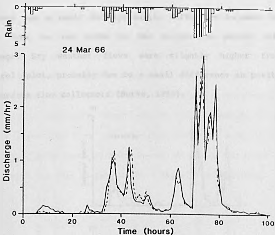
Fig 4.1 Comparison of storm runoff hydrographs from the two experimental plots at Ballinamore in the initial calibration period, prior to drainage.
