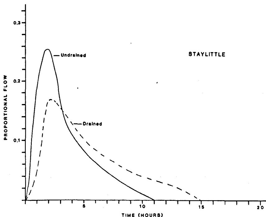
Fig 4.14 Comparison of one-hour average unit hydrographs for storm events before and after drainage at Staylitttle.
