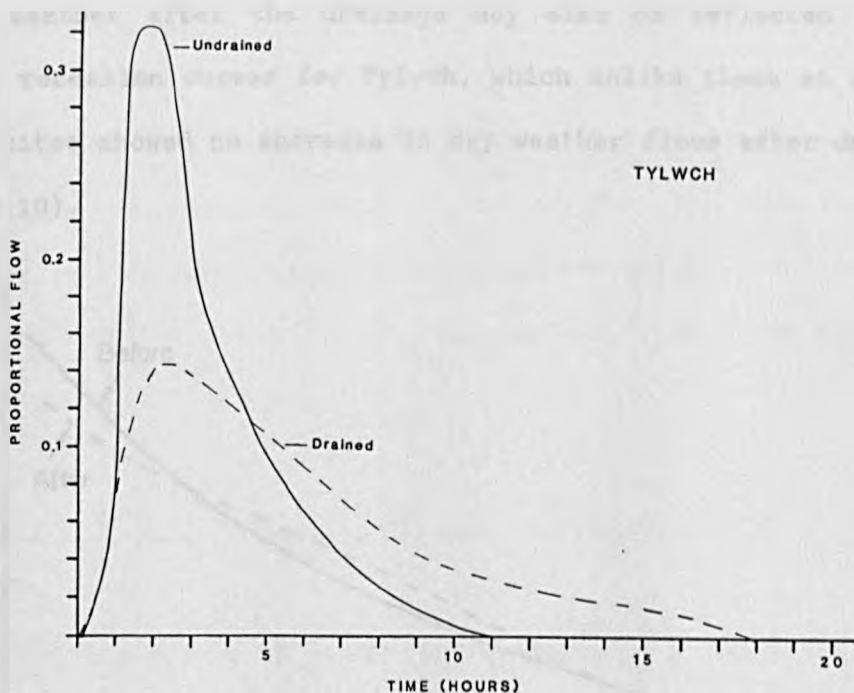
Fig 4.9 Comparison of one-hour average unit hydrographs for periods before and after drainage at Tyllwch.
