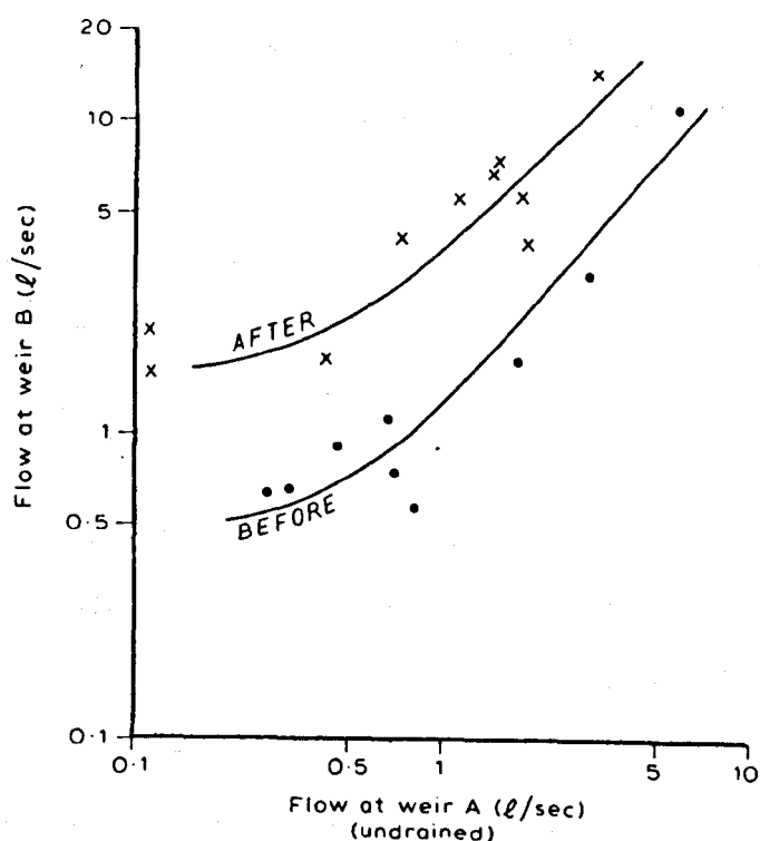
Fig 4.12 Increase in dry weather flows at Witherwick as the percentage of the study area artificially drained was increased from 25% to 56%.
