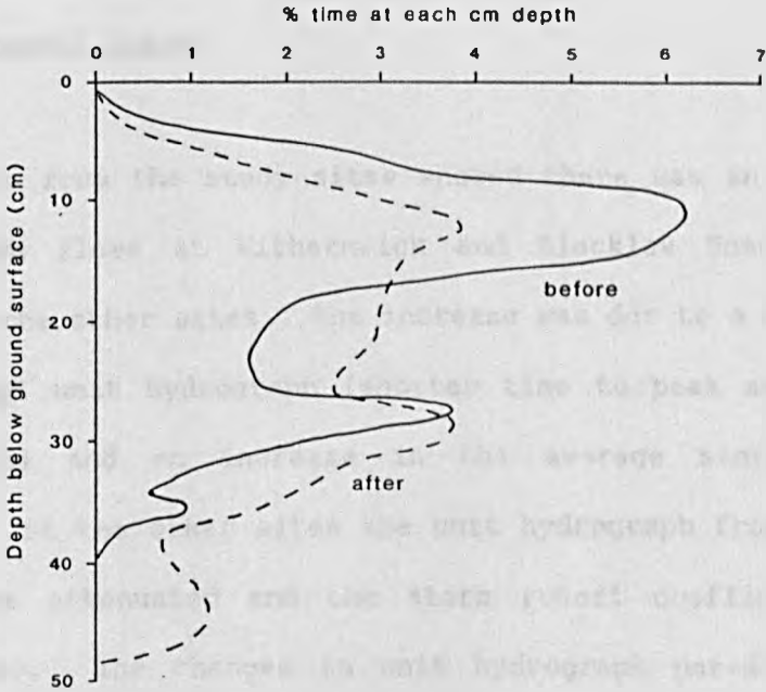
Fig 4.18 Comparison of water table position before and after drainage at Blacklaw Moss.
