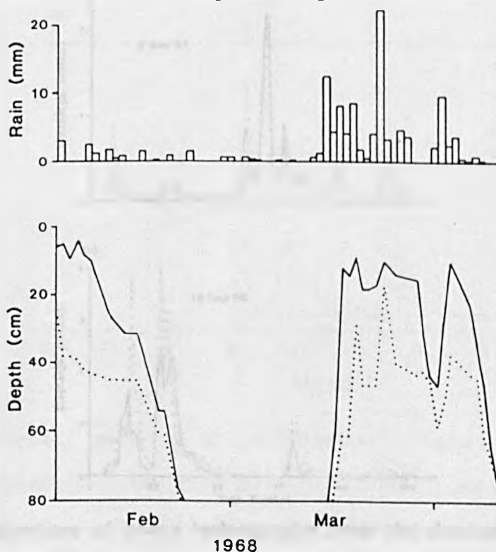
Fig 4.3 Tensiometer data indicate the position of the water table on drained (.....) and undrained (—) land at Ballinamore.
