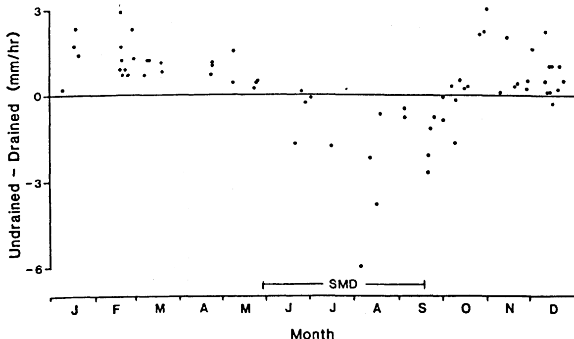
Fig 4.5 Seasonal pattern of differences (mm/hr) in storm hydrograph peaks (undrained minus drained) at Ballinamore. The drained land has lower peak outflows in winter and higher peaks in summer.
