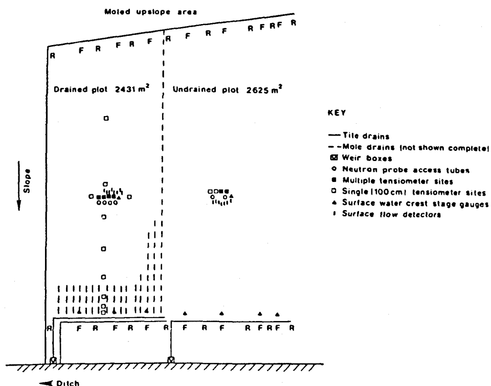
Fig 3.5 Grendon field drainage experiment showing the study site and instrumentation.
