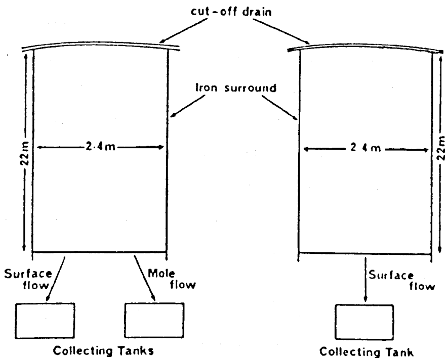
Fig 3.4 Ballinamore field drainage experiment showing the study site and instrumentation.
