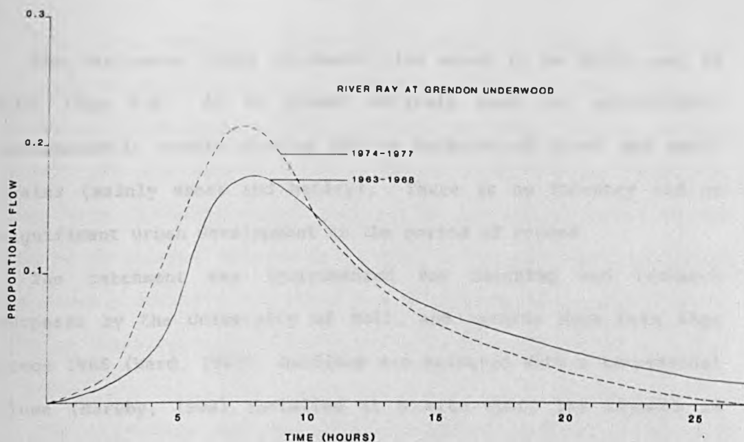
Fig 7.4 Average one-hour unit hydrographs for the Ray showing the effect of field drainage on runoff response.
