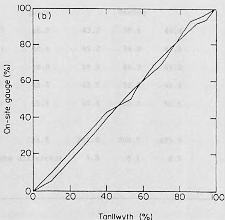
Fig 3.10 Comparison of recorded storm profiles at the onsite gauge at Staylitttle and at Tanllwyth.
