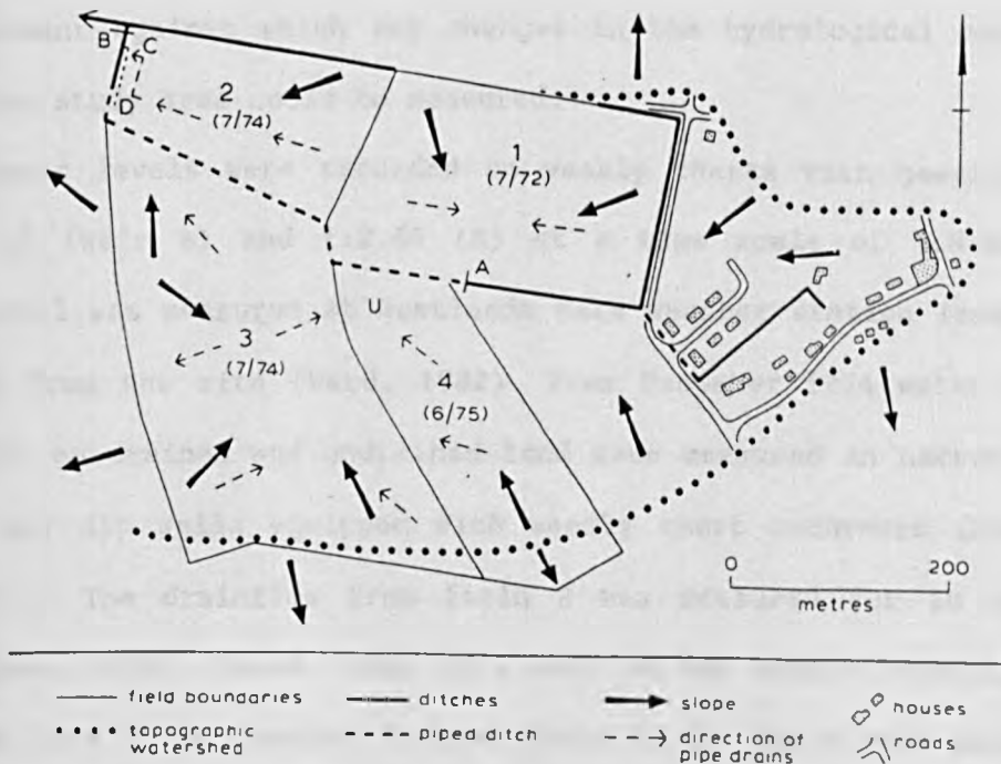
Fig 3.8 Witherwick field drainage experiment showing the study site and instrumentation.
