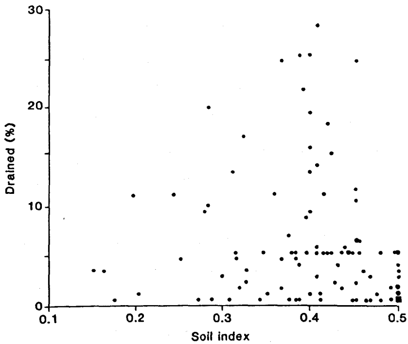
Fig 8.4 Relation between the percentage of drained land and soil index (0.1 = permeable, 0.5 = impermeable).
