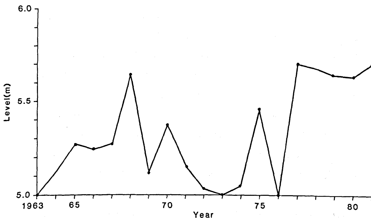
Fig 6.1 Peak stage levels of the river Witham in Lincoln, recorded at the Bargate sluice.
