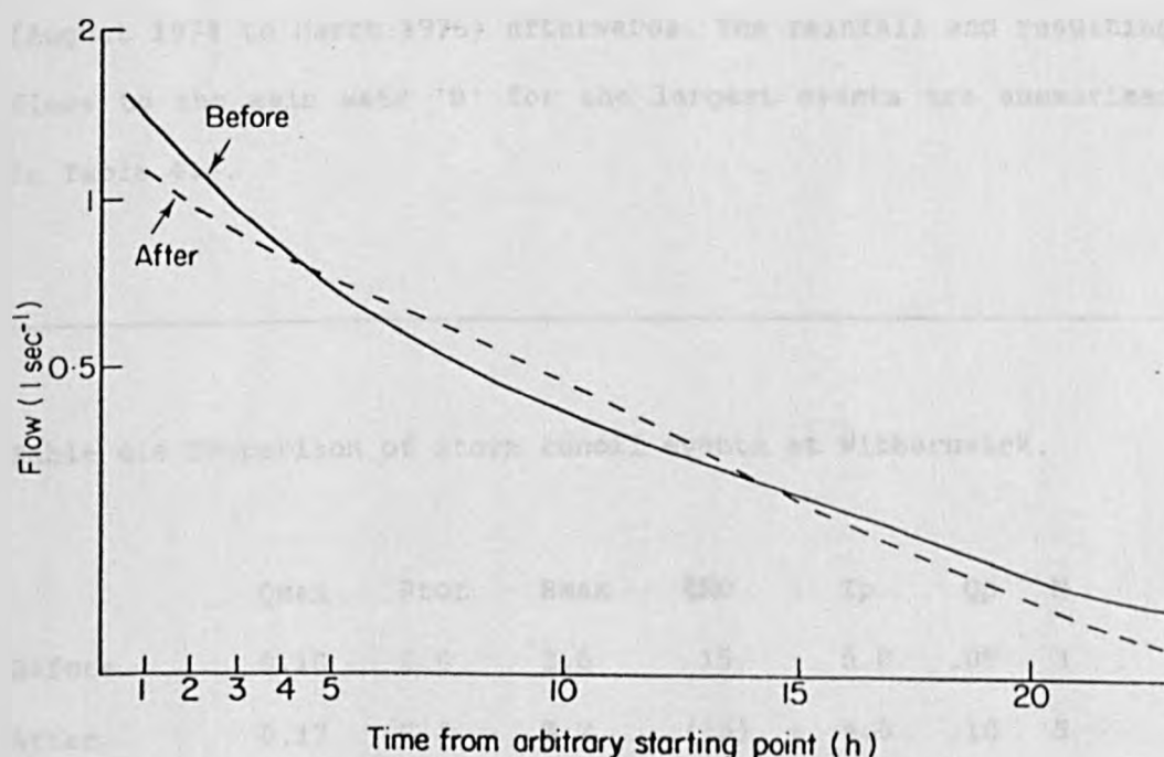
Fig 4.10 Comparison of master recession curves for Tylwch, before and after drainage.
