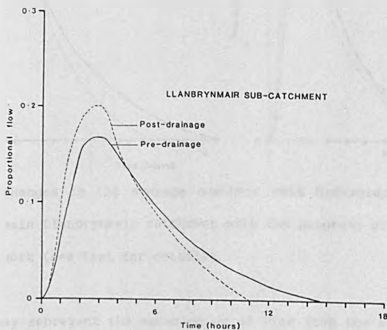
Fig 7.11 Average one-hour unit hydrographs for storm events before and after drainage of the Llanbrynmair subcatchment.
