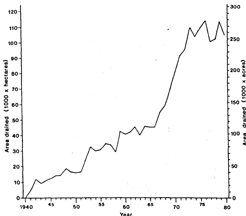
Fig 2.1 Annual area of grant-aided underdrainage in England and Wales, 1940-80.
