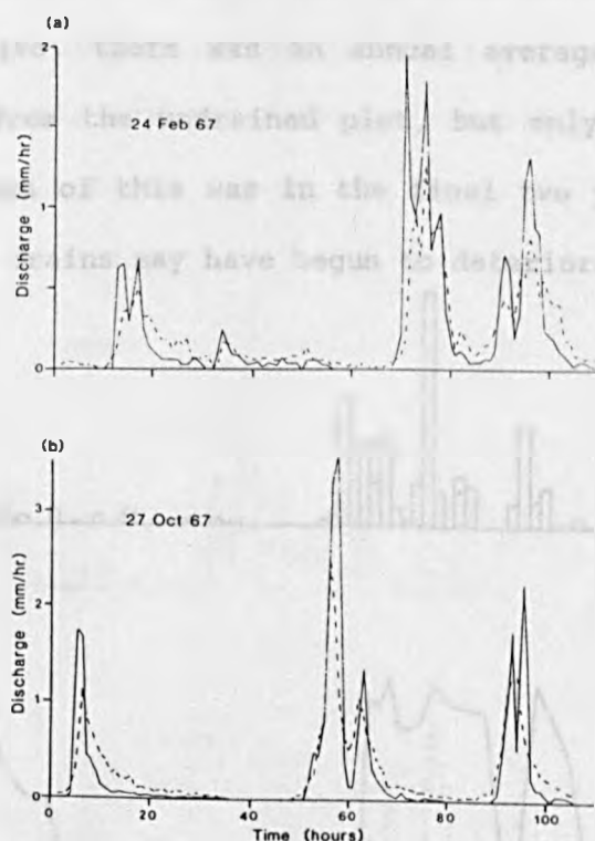
Fig 4.2 Comparison of storm hydrographs from the drained (---) and undrained (—) plots at Ballinamore in a) first winter after drainage b) subsequent winter
