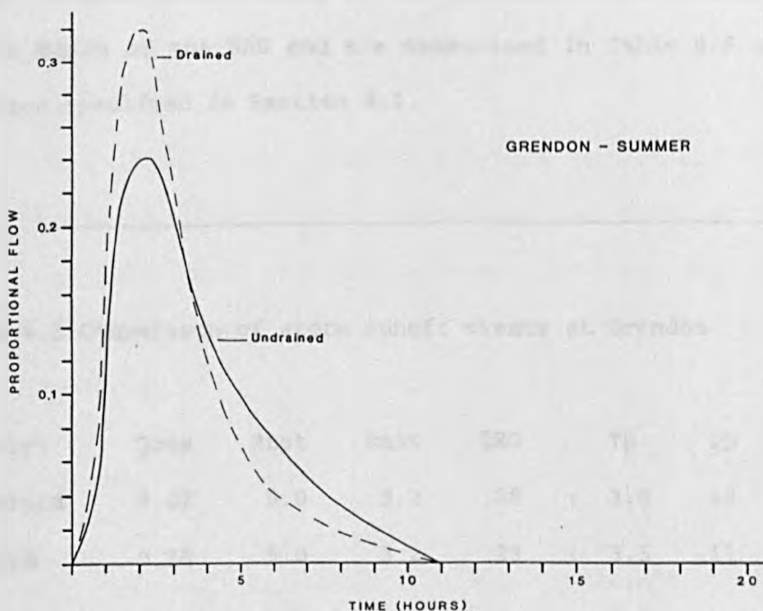
Fig 4.8 Comparison of one-hour unit hydrographs from drained and undrained land at Grendon for summer storms on dry ground (SMD > 5 mm).
