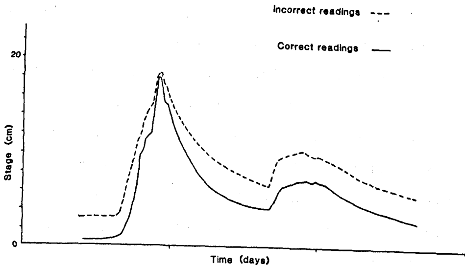
Fig 3.12 Comparison of true and recorded water levels due to a wiring error in the potentiometers used at the Grendon field drainage site.
