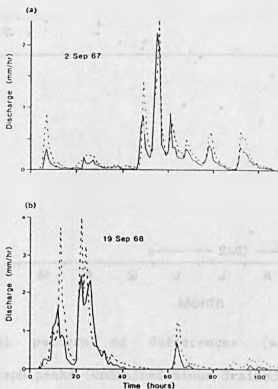
Fig 4.4 Comparison of storm hydrographs from the drained (---) and undrained (—) plots at Ballinamore in a) summer 1967 and b) summer 1968.
