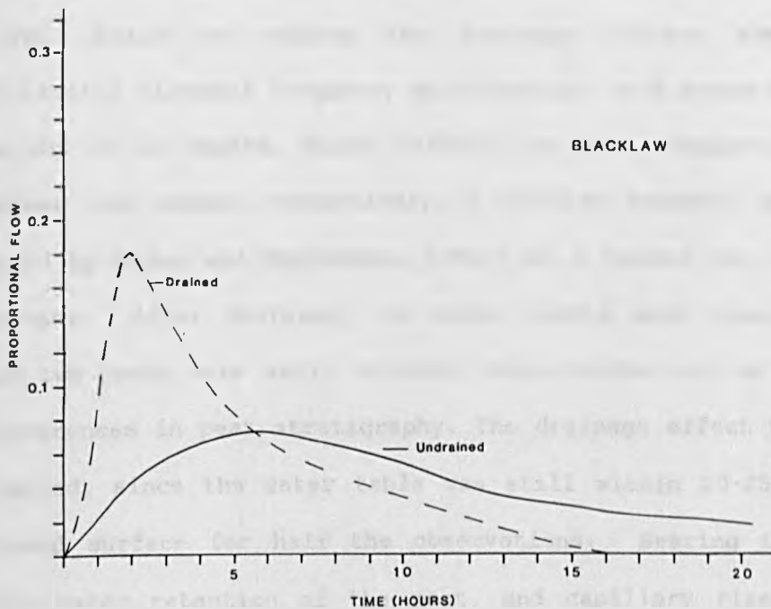
Fig 4.16 Blacklaw Moss one-hour average unit hydrographs.
