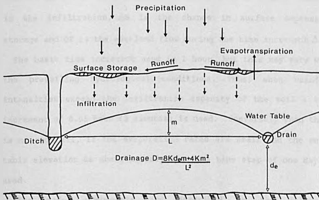
Fig 5.1 Main components dealt with by DRAINMOD
