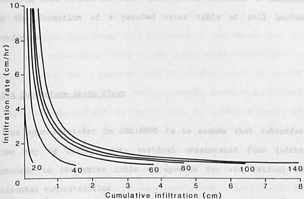
Fig 5.3 Decline in the infiltration capacity of a sandy loam soil initially drained to equilibrium at various initial water table depths (from Skaggs, 1981).
