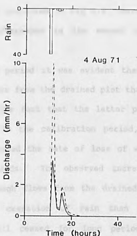
Fig 4.6 Comparison of the outflow hydrographs from drained (---) and undrained (—) land at Ballinamore due to a very intense storm on dry ground in August 1971.
