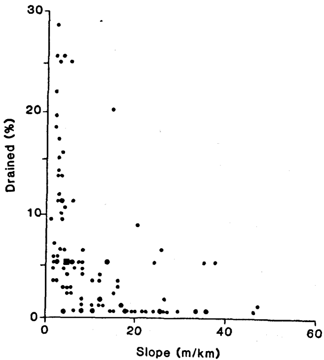
Fig 8.3 Relation between the percentage of drained land and main channel gradient.
