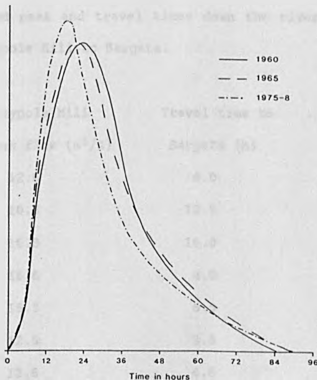
Fig 6.6 Average three-hour unit hydrographs at Claypole, showing the increase in flow response over time.
