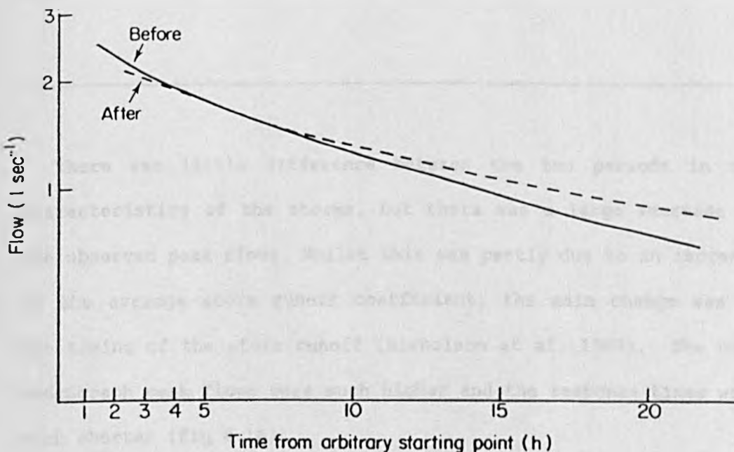
Fig 4.15 Master recession curves for Staylitttle, before and after drainage.
