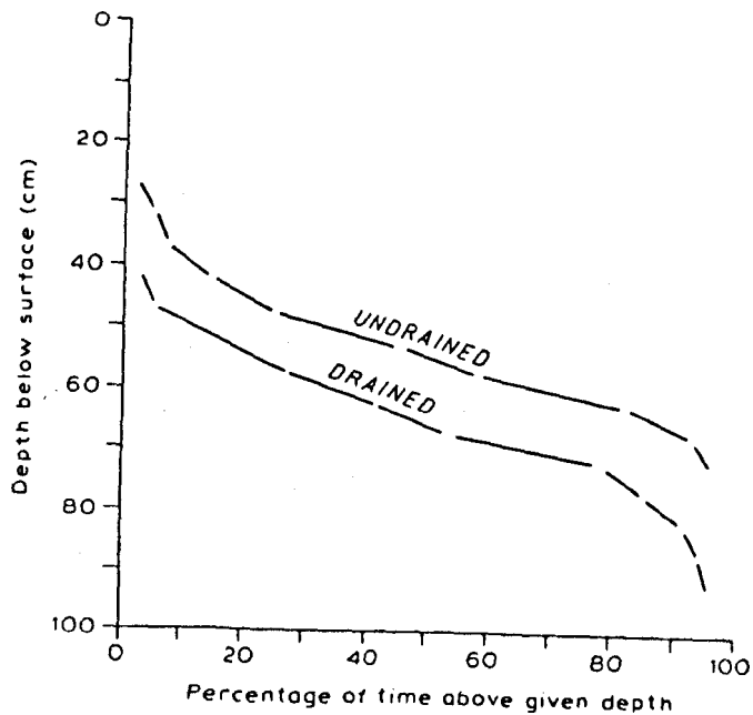
Fig 4.13 Soil water levels in drained and undrained land at Withernwick.
