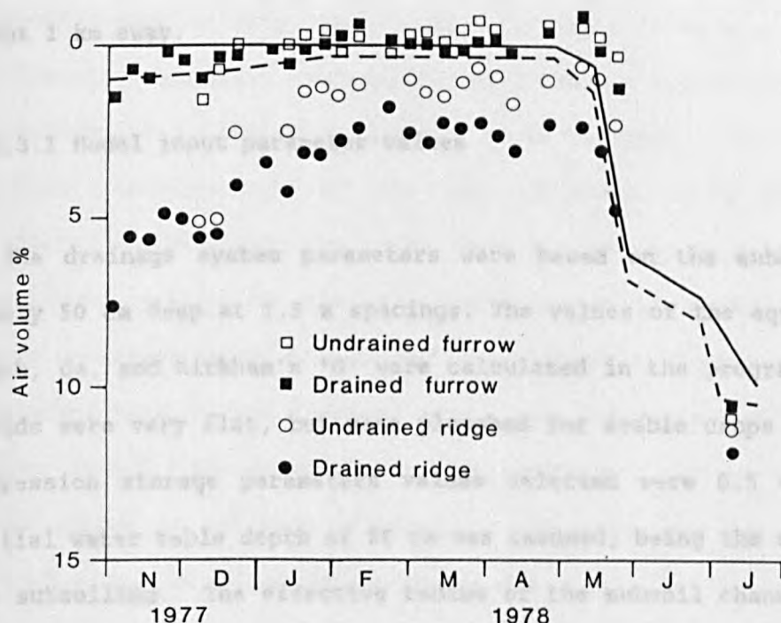
Fig 5.5 Comparison of measured water content at Grendon using a neutron probe with DRAINMOD predictions of the air-filled porosity for drained (---) and undrained (—) land.
