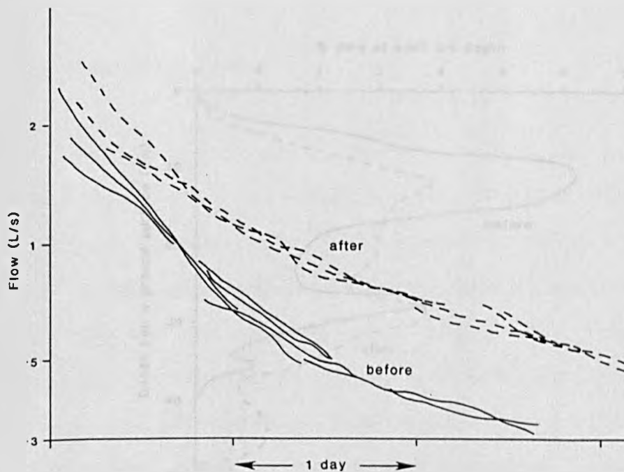
Fig 4.17 Master recession curves for Blacklaw Moss.
