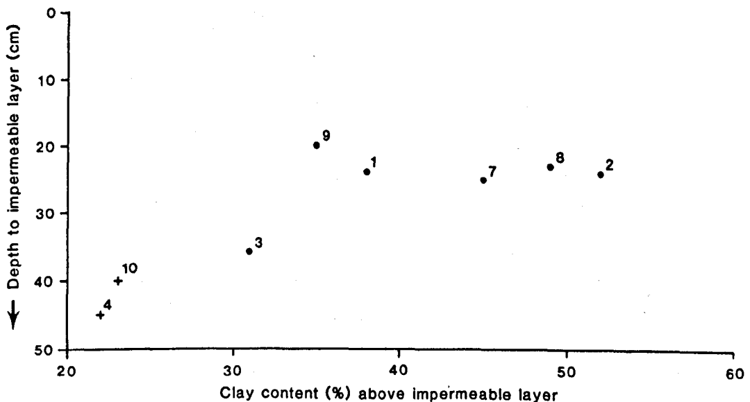
Fig 4.20 Depth to a slowly permeable horizon and the clay content of overlying layers, at sites where drainage increased storm discharge peaks (+) and reduced them (•).
