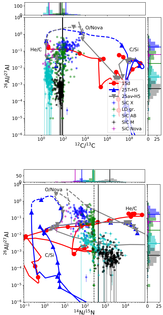
Figure 10. Top Panel: {}^{26}\text{Al}/{}^{27}\text{Al} and {}^{12}\text{C}/{}^{13}\text{C} isotopic ratios predicted from 15d, 25T-H5, and 25av-H5 are compared with SiC grains (178 sub-types AB, 15 nova, and 106 X) and 173 LD graphites. The presolar grains data are available from Hynes & Gyngard (2009) and Stephan et al. (2020). As a reference, we also show the data for 185 SiC mainstream grains (labelled as M), which are the most abundant type of SiC presolar grains and they are made in asymptotic giant branch stars (Zinner 2014, and references therein). The median {}^{26}\text{Al}/{}^{27}\text{Al} ratios are 0.1740, 0.0028, 0.0620, and 0.0006 for SiC-X, AB, Nova, and Mainstream, respectively. The median value for LD graphites is 0.0184. Continuous lines on the main plot represent the He/C and C/Si zones, while the dashed lines indicate the O/nova zone between them. The histograms on the axes show the distribution of each grain type in their respective isotopic ratio, with a solid opaque line indicating the median ratio. Bottom panel: the same as in the top panel, but for {}^{26}\text{Al}/{}^{27}\text{Al} and {}^{14}\text{N}/{}^{15}\text{N} isotopic ratios. Both solar and terrestrial N ratios are shown, as in Fig. 4.
