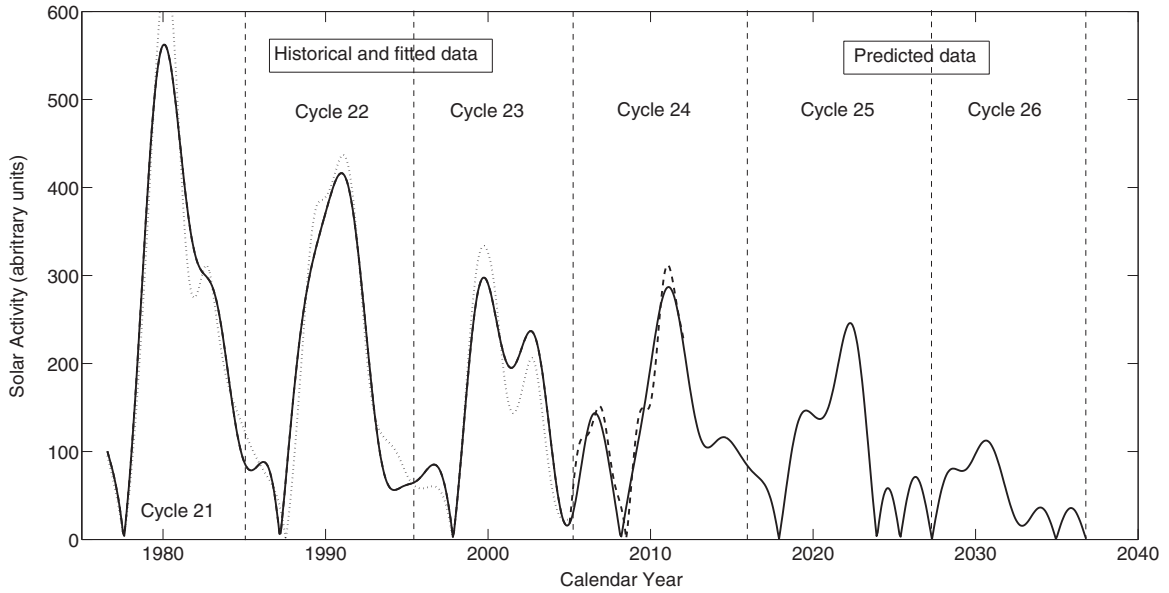
Figure 4. Modulus summary principal component (solid curve) calculated from Equations (6) and (7) for cycles 21–23 and predicted for cycles 24–26, the modulus summary PC derived from SBMF in cycles 21–23 (dotted curve) and in cycle 24 (dashed curve).
