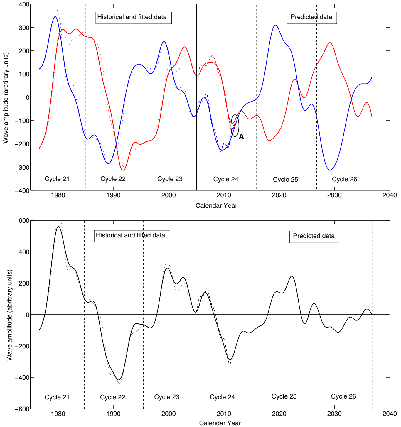
Figure 2. Top plot: the accuracy of the fit with distilled laws from Eureka (solid curves) to the two principal components (PCs) of SBMF (dotted curves) from Figure 1 for cycles 21–23 and their further expansion to cycles 24–26. Bottom plot: the fit of the Eureka -distilled law (the solid curve) to the summary component in cycles 21–23 (dotted curve) and its expansion to cycles 24–26. Dashed curves in both plots show the predicted principal components (top plot) and the summary curve (bottom plot) compared to the real PCs derived from the SBMF in the cycle 24 with an accuracy better than 98%. A letter “A” denotes summer 2014.
