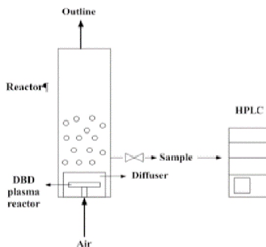
Fig. 1 Process diagram of TPA treatment with ozone in form of microbubble
