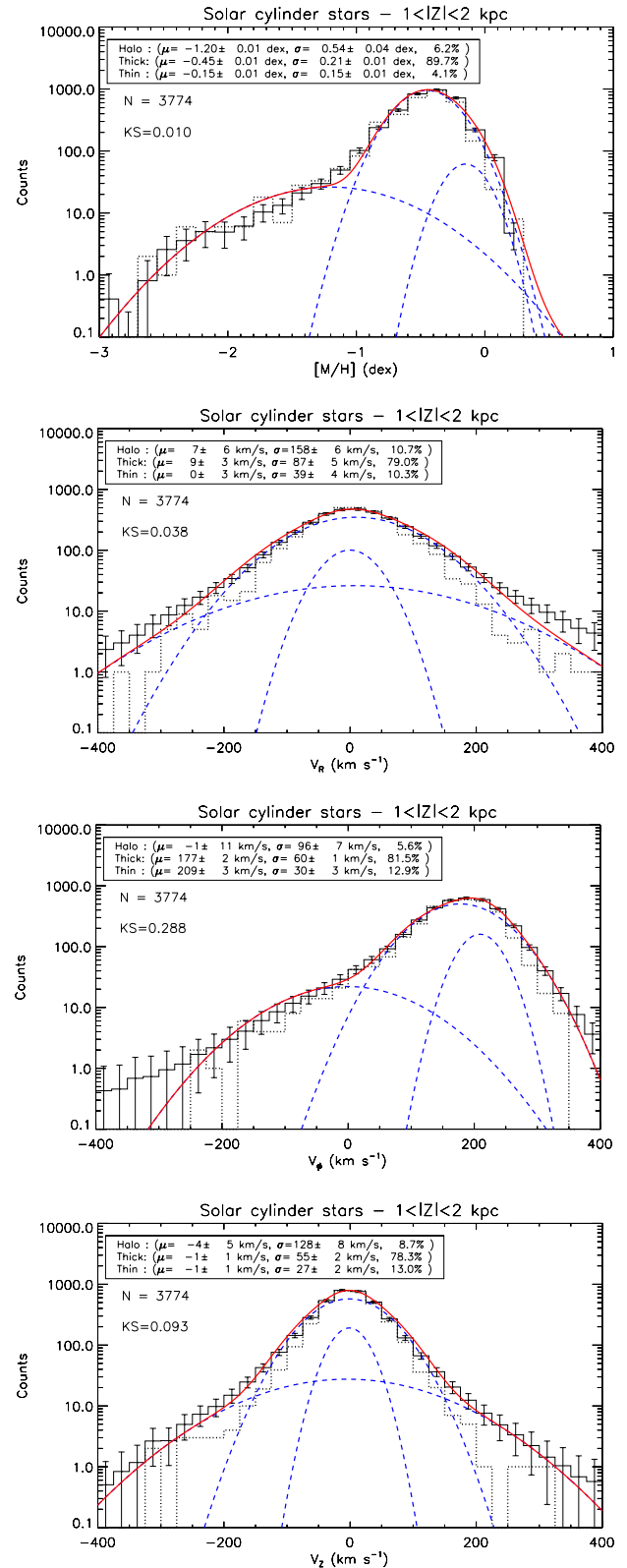
Figure 6. Metallicity ( [M/H] ), orbital Galactocentric radial velocity ( V_R ), orbital azimuthal velocity ( V_\phi ) and orbital vertical velocity ( V_z ) distributions in the solar cylinder for all the stars between 1 kpc and 2 kpc away from the Galactic plane. The colour coding is the same as in Fig. 4.
