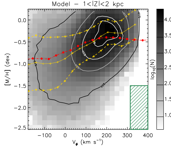
Figure 8. Same as the middle panel of Fig. 7, but for our simple three-component Gaussian model. The red curve represents the result obtained from the observations, i.e. the one from the middle panel of Fig. 7.
