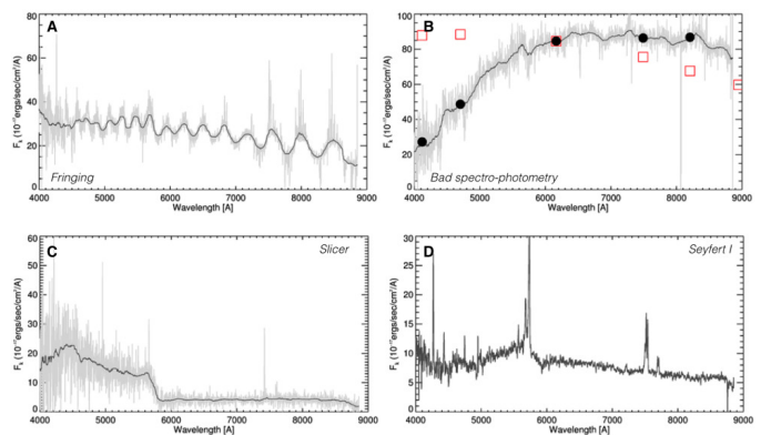
Fig. 3. Example spectra representing our four quality flags. Panel A) shows an example of a fringed spectrum. A spectrum with failed spectro-photometry is shown in panel B), wherein the red open squares are the fluxes estimated from the SDSS photometry inside the fibre aperture. Panel C) shows a spectrum with clear splicing problems around observed frame 5700 \text{ \AA} , where the blue and red spectra have been unsuccessfully joined. An example spectrum with broad hydrogen emission lines classified as Seyfert I is shown in panel D).
