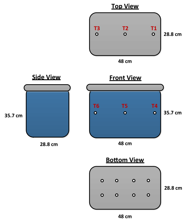
Fig. 1 Bioreactor design
