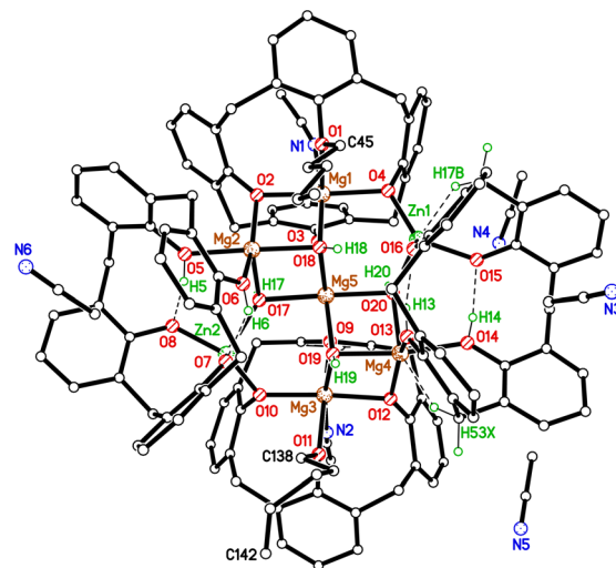
Fig. 4 Two views of the molecular structure of [Mg_5Zn_2(OH)_4(LH)_2]^{2-} ( (LOpenty)_2(NCMe)_2 )]·5MeCN ( 4-5MeCN ) ( tert -butyl groups & most H atoms omitted for clarity). Selected bond lengths (Å) and angles ( ^\circ ): Mg(1)–O(1) 2.141(17), Mg–(non-alkylated calixarene O) range 1.937–2.073(17), Mg(1)–O(18) 2.033(15), Mg(1)–N(1) 2.20(2), Mg(2)–O(17) 1.994(15), Mg(2)–O(18) 2.053(13), Mg(5)–O(17) 2.081(15), Mg(5)–O(18) 2.145(14), Mg(5)–O(19) 2.114(16), Mg(5)–O(20) 2.083(17), Zn–(non-alkylated calixarene O) range 1.862–1.935(18), Zn(1)–O(20) 1.981(15); Mg(1)–O(2)–Mg(2) 97.5(7), Mg(1)–O(18)–Mg(5) 98.0(7), Mg(2)–O(17)–Mg(5) 97.6(7), Mg(3)–O(12)–Mg(4) 98.6(6), Mg(3)–O(9)–Mg(5) 101.7(9), Mg(2)–O(17)–Zn(2) 120.7(8), Mg(3)–O(10)–Zn(2) 119.3(8), Mg(4)–O(19)–Mg(5) 94.6(6), Mg(1)–O(4)–Zn(1) 114.0(7).
