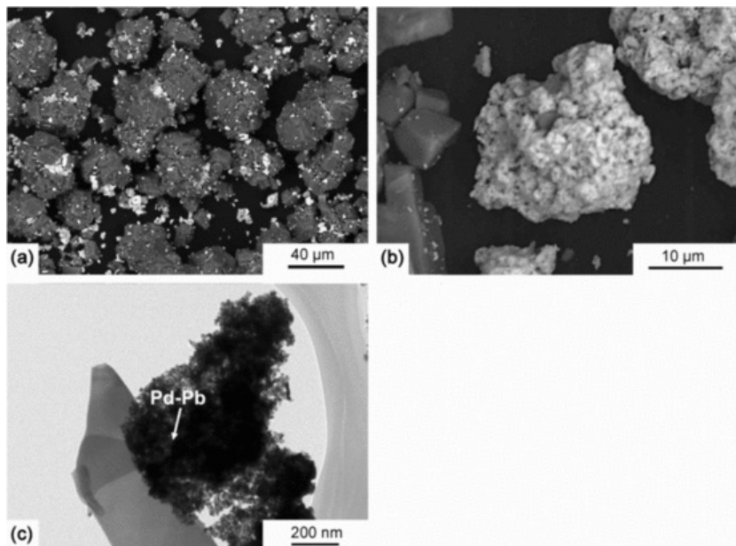
Fig. 3 (a, and b) SEM and (c) TEM microphotographs of the Lindlar catalyst.
