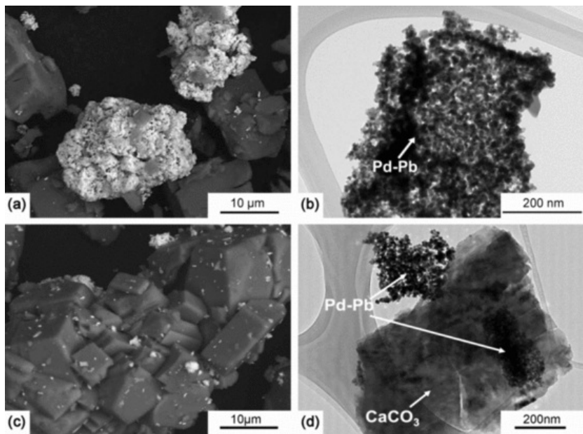
Fig. 4 Representative SEM and TEM microphotographs of the (a and b) Lstir catalyst used in the hydrogenation with the conventional stirring, and (c and d) L40 US-treated catalyst at 40 kHz. Pd-Pb particles on TEM study were confirmed by EDX analysis.
