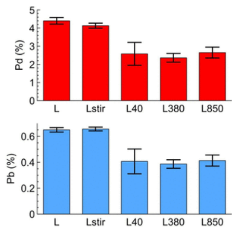
Fig. 2 Pd and Pb content (wt %) retained on the Lindlar catalysts after the hydrogenation for 2.5 h at 40, 380, 850 kHz US frequencies (L40, L380, L850, respectively), in comparison to the original Lindlar catalyst (L) and the catalyst after the reaction with the conventional stirring (Lstir).
