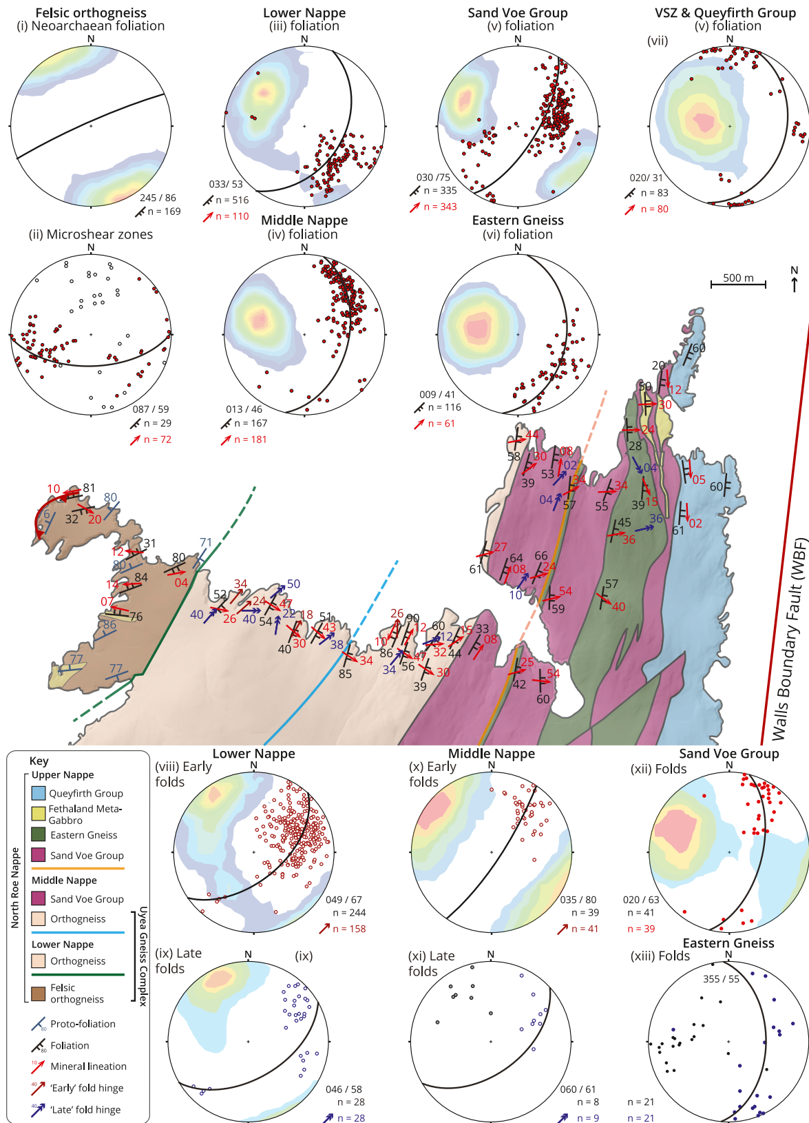
Fig. 3. (a) Geological map of North Roe showing foliation and lineations measurements. Stereonets display pole-to-plane contoured foliation, lineation and mean foliation plane (using right hand rule) for (i) 'Neoarchaeon' foliation in foliated granodiorite; (ii) microshear zones in the Foliated granodiorite; (iii) Lower North Roe Nappe; (iv) Middle North Roe Nappe orthogneiss; (v) Sand Voe Group; (vi) Eastern Gneiss; (vii) VSZ and the Queyfirth Group. Stereonets viii-xiii display pole-to-plane contoured axial planes, fold hinges and mean axial plane for (viii) 'Early' folds in Lower North Roe Nappe, (ix) 'Late' folds in Lower North Roe Nappe, (x) 'Early' folds in Middle North Roe Nappe, (xi) 'Late' folds in Middle North Roe Nappe, (xii) Sand Voe Group, (xiii) Eastern Gneiss.
