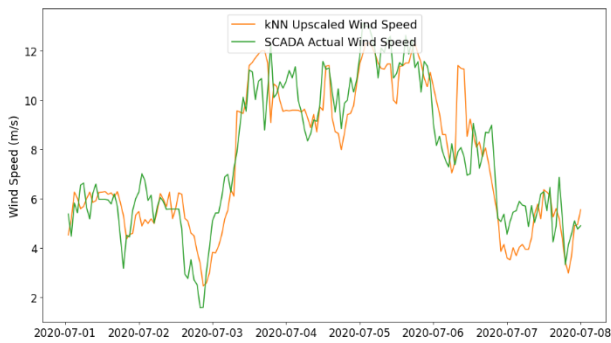
Fig. 4. 1-week wind speed prediction (Q2 2019 training)
