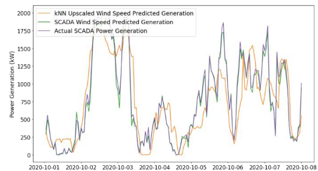
Fig. 9. 1-week 2020 power prediction (Q3 2019 training)
