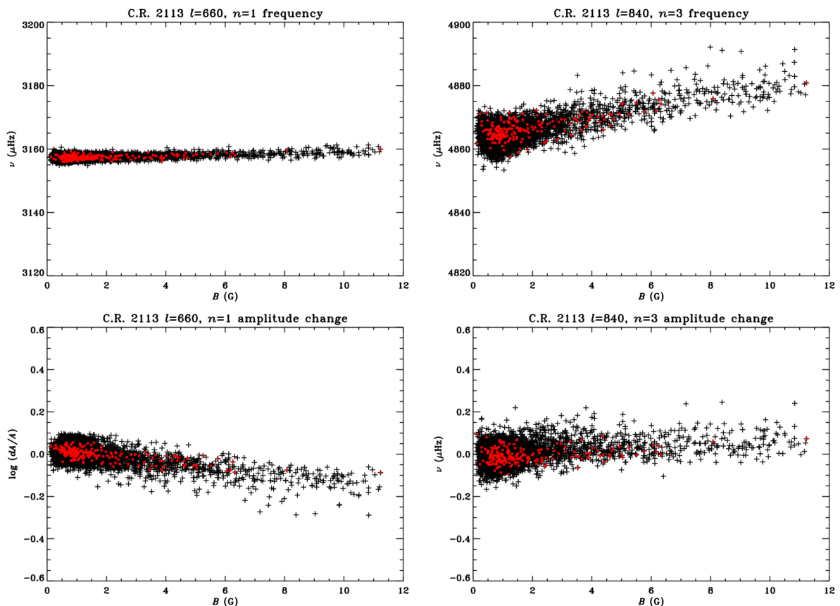
Figure 4. Scatter plots of frequency (top) and amplitude (bottom) change against MAI for low-activity regions in C.R. 2113. The red symbols represent patches in the coronal hole areas and the black symbols other patches in the same MAI range, for sample peaks in the 5-min band (left) and at the acoustic cutoff (right). Both sets of data are restricted to latitudes below 50 degrees.
