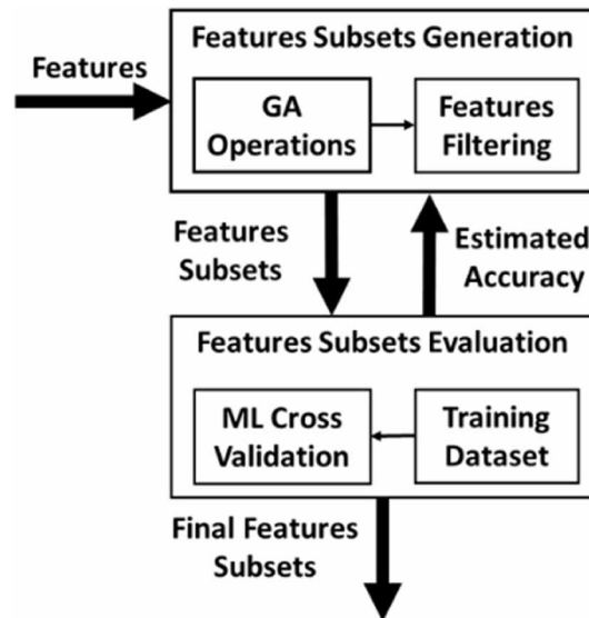
Figure 8. GA feature subsets selection as Wrapper Approach
