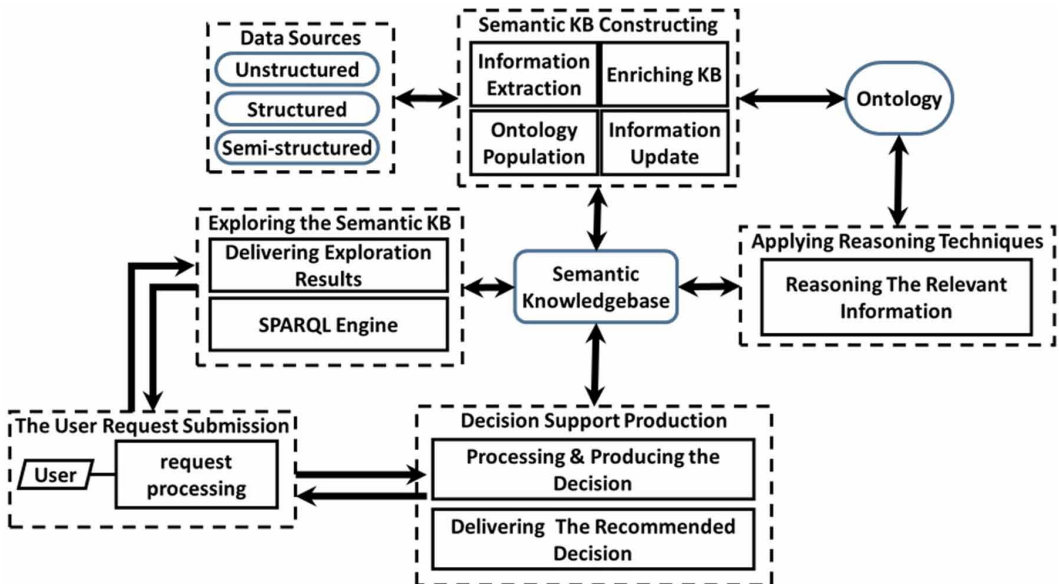
Figure 10. The main components of exploring semantic knowledgebase and the integrated Decision Support System
