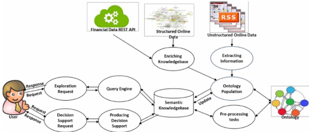
Figure 1. The overview of the framework implementation scenario
