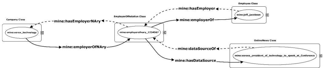
Figure 6. Inverse N-ary Relation Example
