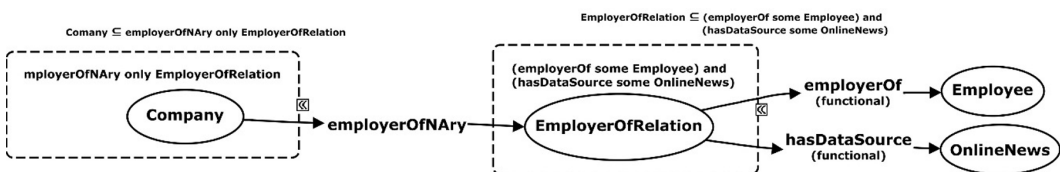
Figure 7. OWL axioms for N-ary relations example
