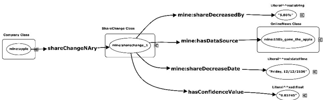
Figure 5. N-ary Relation Example
