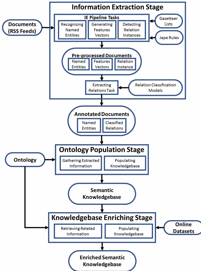
Figure 9. The process of constructing semantic knowledgebase stages
