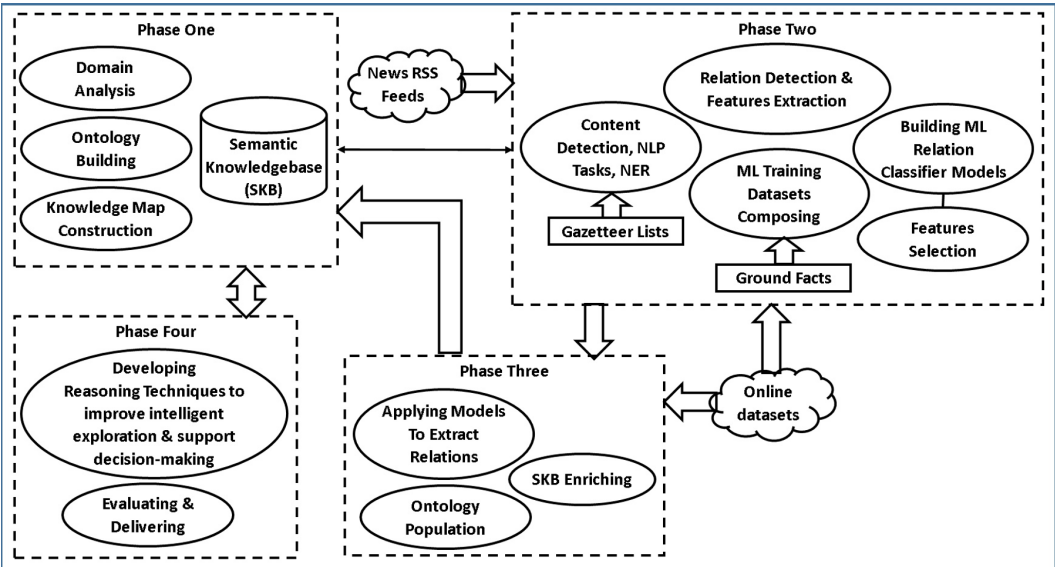
Figure 2. The Concept Map sample of the problem domain of this work
