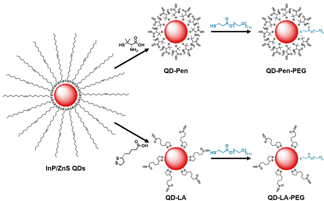
Fig. 1 Preparation of QD formulations. Schematic of the synthetic procedures for preparation of QD-Pen, QD-LA, QD-Pen-PEG, and QD-LA-PEG from InP/ZnS QDs. Please note, ligand numbers and ratios are not representative.
