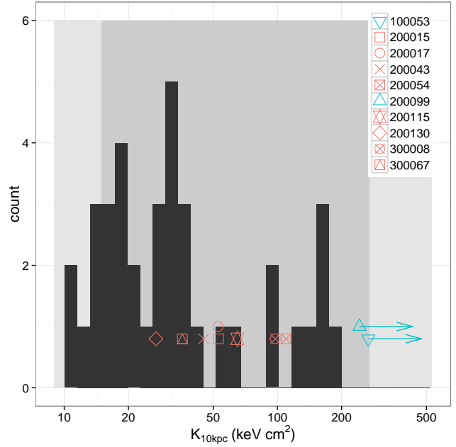
Figure 4. Histogram of group entropies at 10 Kpc using the entropy profiles of the ACCEPT sample (Cavagnolo et al. 2009) with k_B T < 3 keV with our measured entropies overlaid. As in Figure 3 we show the 1\sigma ( dark shading ) and 2\sigma ( light shading ) upper and lower limits at 10 kpc derived from the OWLS simulations (McCarthy et al. 2011).
