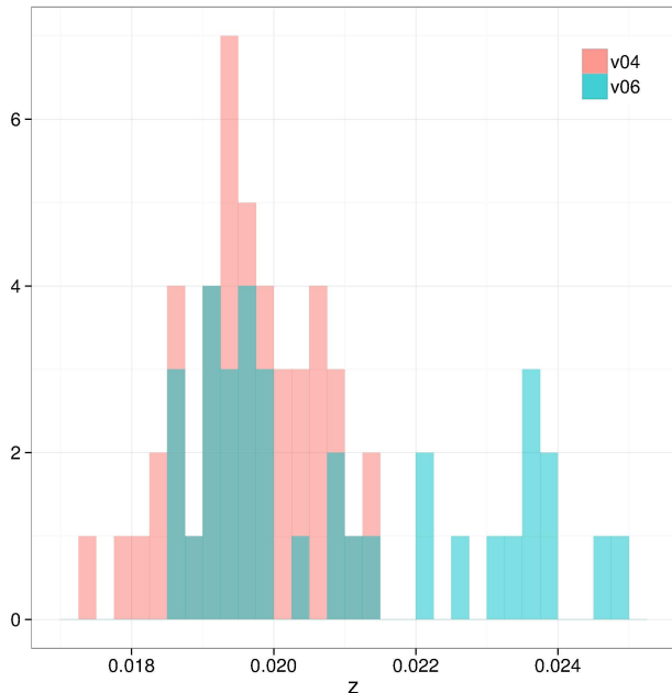
Figure 6. Histogram of galaxy redshifts for members of group 200130 (MKW4) identified within G3Cv04 (red) and G3Cv06 (blue) group catalogues. A large fraction of the galaxies linked to this group in G3Cv04 are part of another group in G3Cv06 (see text and Section 2.4).
