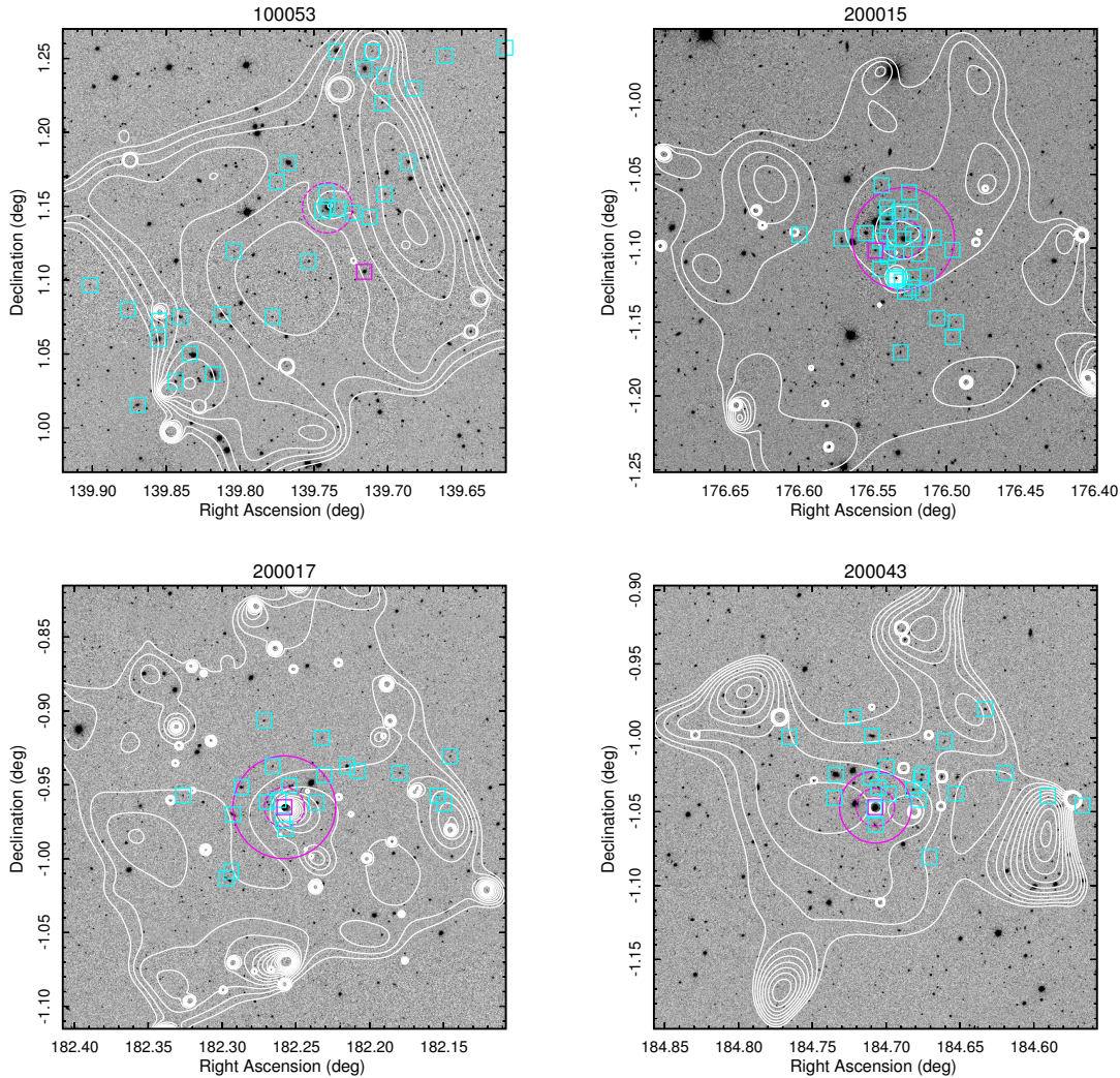
Figure 1. Optical images of our groups from the SDSS with X-ray contours overlaid ( white lines ). The X-ray contours are derived from adaptively smoothed images of the observed X-ray emission in our analysis band (0.3–3.0 keV) set at arbitrary levels for illustration purposes only. Also shown are the G3Cv06 member galaxies ( cyan squares ) with central galaxies (as defined by our iterative centre of light algorithm defined in Section 2.5) marked by magenta squares . For scale we illustrate a 100 kpc region with a dashed magenta circle and the extraction region, when different, by the solid magenta circle centred on the X-ray source to be analysed (either the X-ray centroid or an optical centre, Section 2.5).
