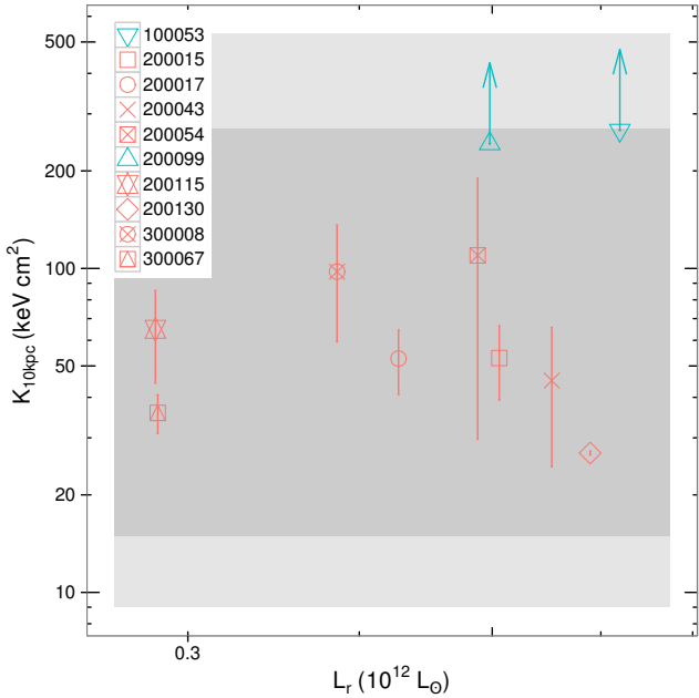
Figure 3. Central (10 kpc) entropies against total optical r -band luminosity. We show the 1\sigma ( dark shading ) and 2\sigma ( light shading ) upper and lower limits at 10 kpc derived from the OWLS simulations (McCarthy et al. 2011).
