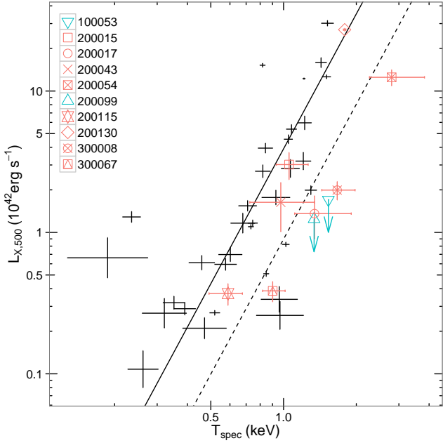
Figure 2. The luminosity – temperature relation for our group sample ( coloured points ). Overlaid are groups from the Osmond & Ponman (2004) sample ( black points ). The solid line represents the L - T relation of Slack & Ponman (2014). We show the L - T relation of our sample, modified from the Slack & Ponman (2014) relation by refitting the normalisation only, excluding the undetected groups 100053 and 200099, as the dashed line .
