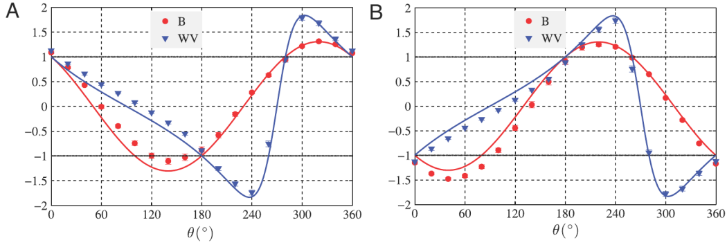
Figure 6. (Color online) Results from the optics experiment of Ref. [22], which show the Leggett-Garg parameter (labelled B, red) and a weak value (labelled WV, blue) for a range of input states parametrized by the angle \theta . The two parts show results for different measurements at the second position in the three-measurement experiment, with solid lines showing the theoretical predictions and points, the experimental data. It is evident that for this 3-point LGI test with semi-weak measurements, a violation of the LGI is accompanied by the emergence of a weak value. The measurement strength here was K = 0.5445 \pm 0.0083 . The experiment was repeated with K = 0.1598 \pm 0.0091 and larger LGI violations were observed. Figure from Goggin et al. [22].
