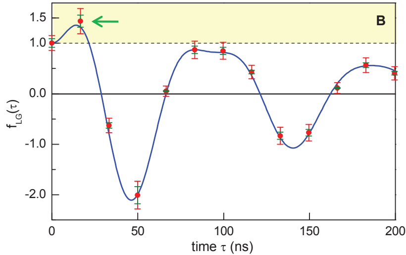
Figure 3. (Colour online) Experimental results from the measurement of the three-term continuous-weak-measurement Leggett-Garg inequality, Eq. (57), for a superconducting transmon qubit. Red points are experimental data points; the blue line, theoretical quantum prediction and yellow, the region forbidden under Leggett-Garg assumptions. The data point marked with the arrow indicates a violation at short times. Figure from Ref. [11].
