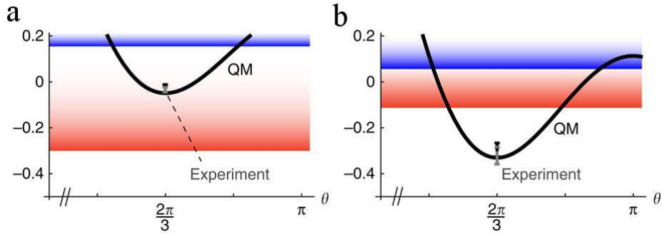
Figure 5. (Color online) Results from the nuclear spin experiment of Ref. [31]. Shown is the LGI correlator f \equiv 1 - K'_3 as a function of the system evolution angle \theta . The black line shows the theoretical prediction and the data point, the experimentally-measured result. With perfect ancilla preparation, a realistic description of the spin implies that f \geq 0 . Taking imperfect preparation into account, the bound on f becomes Eq. (59) with “venality” \zeta the fraction of incorrectly-prepared ancillas, and this is shown in red (blue denotes a less strict bound, not discussed here). The two figures show the results for two initial ensembles: (a) a thermal initial state (2.6 K) and (b) a highly polarized state. For the thermal ensemble, the measured value lies between -2\zeta and zero — this means that the apparent violation of the LGI can be explained away in terms of ancilla errors. For the polarized ensemble, the measured value satisfies f < -2\zeta , such that a genuine violation of the LGI can be claimed. Figure from Ref. [31].
