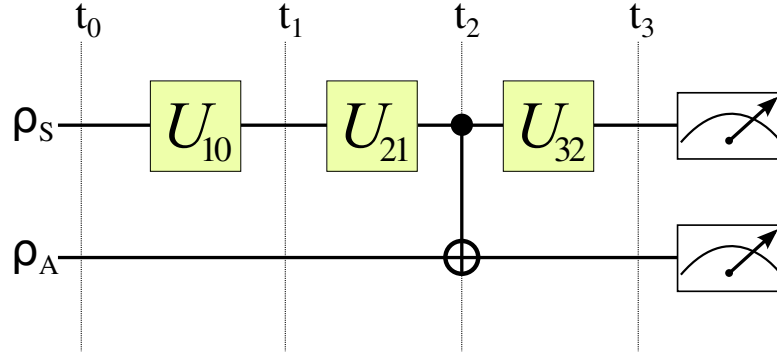
Figure 4. (Color online) Quantum circuit to non-invasively measure part of the correlation function C_{32} . The system qubit is prepared in state \rho_S and the ancilla qubit in \rho_A . The time evolution of the system is induced by the unitary operators U_{ji} acting between times t_i and t_j . The measurement at t_2 is carried out with a CNOT-gate, in which the state of the ancilla is flipped if the system is in the \uparrow -state and left unaltered if the system is in the \downarrow state. The ancilla is then read-out at the end and only results where no flip has occurred are kept. The measurement of the system at t_3 can be performed invasively. This circuit is then repeated with an anti-CNOT gate instead and the measurements combined to build C_{32} from ideal negative measurements. Adapted from Knee et al. [31].
