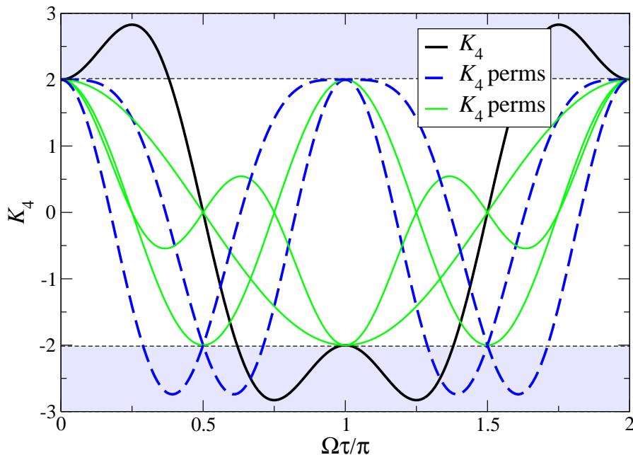
Figure 2. (Color online) Same as in Fig. 1, but here for the fourth-order Leggett-Garg inequality, |K_4| \leq 2 . The thick black curve depicts K_4 itself; the other curves show K_4 with permutations of time indices. Permutations that lead to violations of the inequality are plotted with blue dashed curves, and those that do not, with green thin curves.
