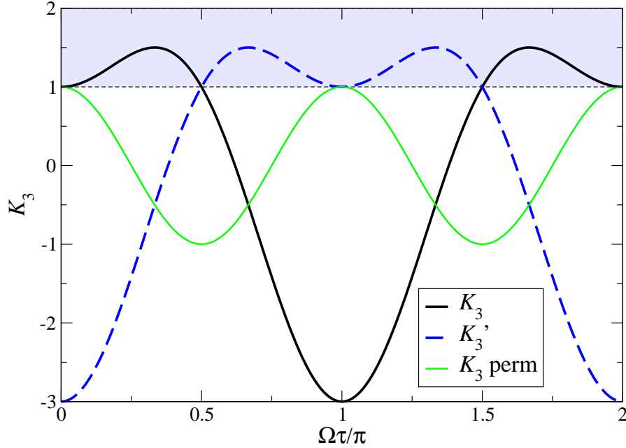
Figure 1. (Color online) Third-order Leggett-Garg function K_3 with equi-spaced measurements for a qubit as a function of measurement-time spacing \tau . The solid black curve shows the quantity K_3 ; the blue dashed curve the quantity K'_3 , and the thin green curve shows the function obtained by permuting the indices of K_3 . The blue shaded region denotes values of K_3 excluded by the Leggett-Garg inequality and thus incompatible with macroscopic realism and non-invasive measurability. A violation of one or the other of the K_3 and K'_3 inequalities occurs for all \tau except at multiples of \pi/2 .
