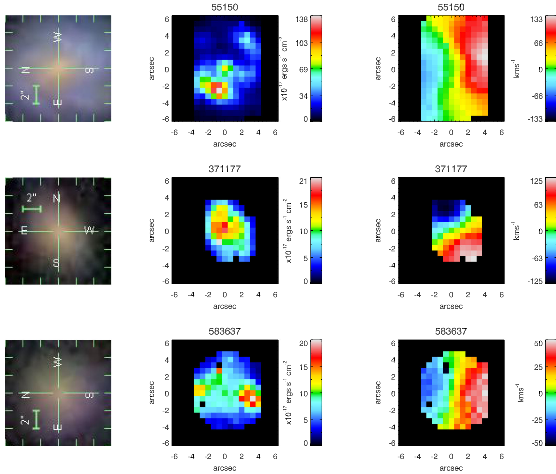
Figure A5. Low-density environment galaxy sample cont. From left to right: SDSS thumbnail image of SPIRAL field of view, H\alpha flux map of central region; H\alpha velocity map of central region. Only spaxels with signal-to-noise ratios >3 are shown.
