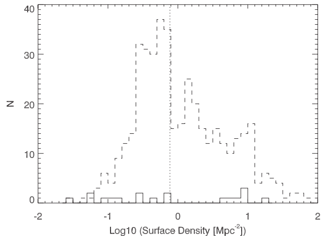
Figure 1. Histogram showing the surface density distributions of the 424 possible targets (dashed line) and the 18 observed galaxies (solid line). The dotted line indicates the median surface density of 0.77\text{ Mpc}^{-2} that divides the low- and high-density samples analysed here. The observed galaxies sample the possible density distribution well and the low- and high-density subsamples can be seen to be well separated.
