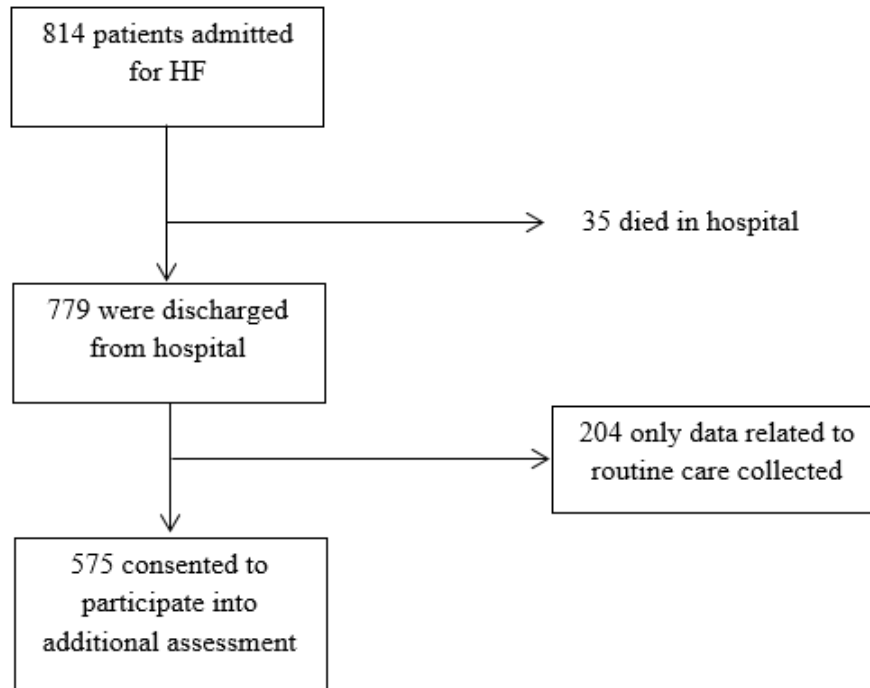
Figure 1 Consort Diagram
