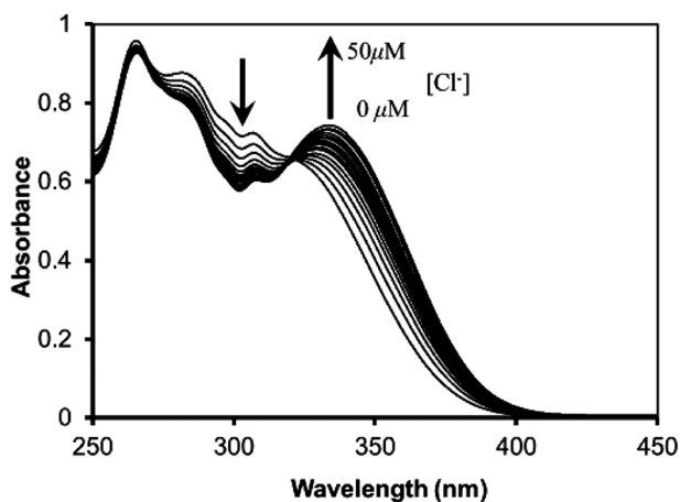
Fig. 2 UV-vis absorption spectra of receptor 4_{\text{e}} (2.5 \mu\text{M} ) upon the addition of Bu 4 NCl (0–50 \mu\text{M} ) in \text{CH}_2\text{Cl}_2 -DMSO (10 : 1, v/v).
