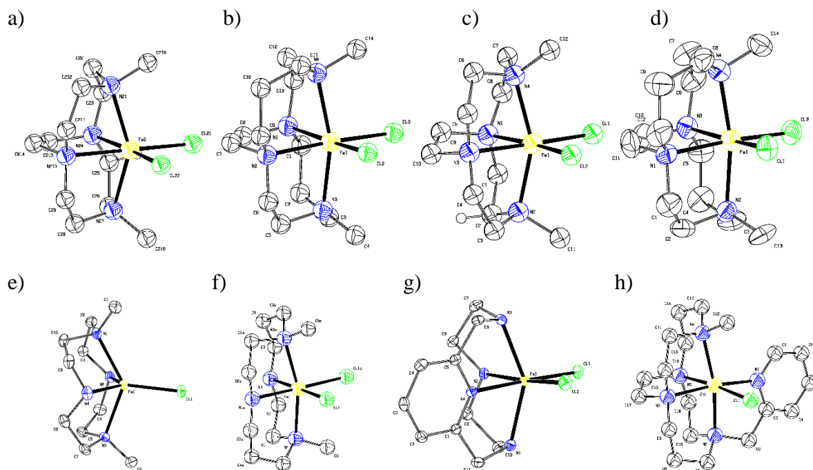
Figure 6. ORTEP (50% TEP) representation of a) [\text{Fe}^{2+}\text{L7}(\text{Cl})_2] b) [\text{Fe}^{2+}\text{L8}(\text{Cl})_2] c) [\text{Fe}^{3+}\text{L7}(\text{Cl})_2]^+ d) [\text{Fe}^{3+}\text{L8}(\text{Cl})_2]^+ e) [\text{Fe}^{2+}(\text{L5})\text{Cl}]^+ f) [\text{Fe}^{2+}(\text{L6})\text{Cl}_2] g) [\text{Fe}^{3+}\text{L1}(\text{Cl})_2]^+ h) [\text{Fe}^{2+}\text{L10}(\text{Cl})]^+ . Hydrogen atoms and counter-ions have been omitted for clarity. 35, 98-99
