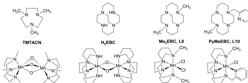
Figure 3. Ligands and catalytically active manganese complexes studied previously. 44-46, 48, 51, 66-
