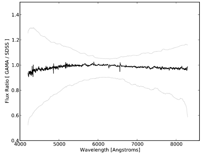
Figure 4. The median ratio of common GAMA and SDSS spectra. This result is derived from 574 objects out of the 637 objects that were observed by both surveys. The 63 spectra excluded were due to particularly noisy GAMA spectra, or redshift mismatches between the surveys. The spectra are first normalized by the median flux value of the flux-calibrated spectrum (since the absolute flux calibration is scaled differently between GAMA and SDSS). The spectra are then median filtered by 7 \text{ \AA} and interpolated to the same wavelength scale before the ratio was taken. The dark line shows the median of the flux ratios, and the outer, grey lines show the 68th percentile range of the distribution of ratios for individual objects.
